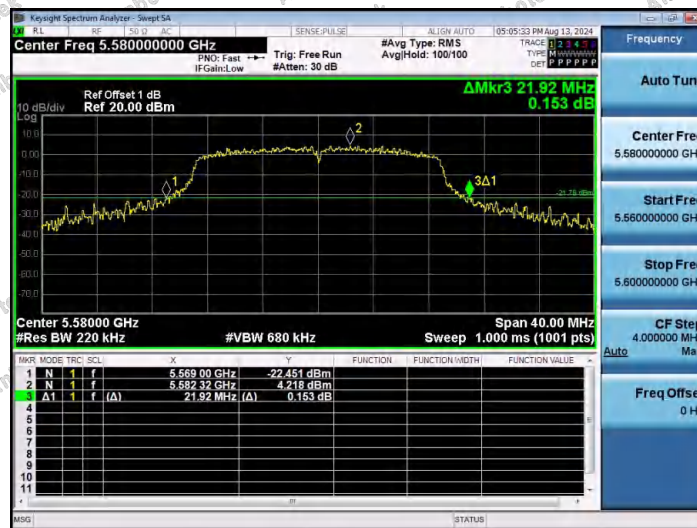
11N20SISO-Ant1-5580
