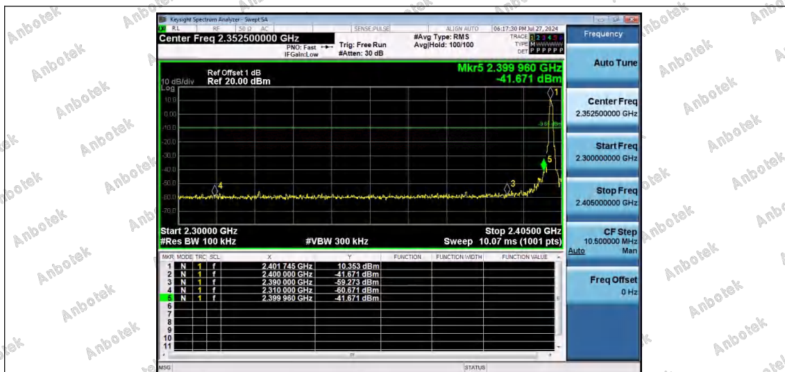
BLE_1M-Ant1-2402-PASS
