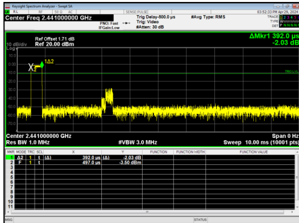
Burst(2DH1)
