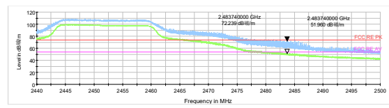
802.11g-Channel 9 Peak+ Average
