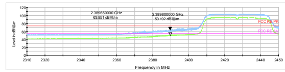
802.11n HT40 -Channel 4 Peak+ Average
