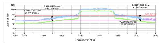
802.11n HT40 -Channel 6 Peak+ Average
