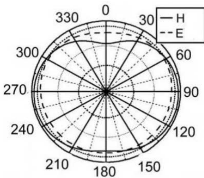
49.86MHz radiation pattern
