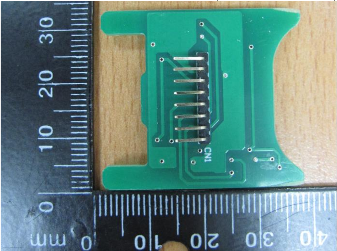
Figure 10 Internal View (Control Board, Front View)
