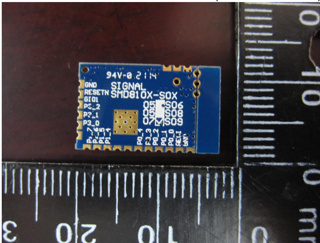
Figure 14 Internal View(RF Module/Back View)
