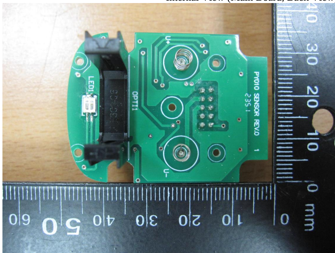
Figure 12 Internal View (Main Board, Back View)
