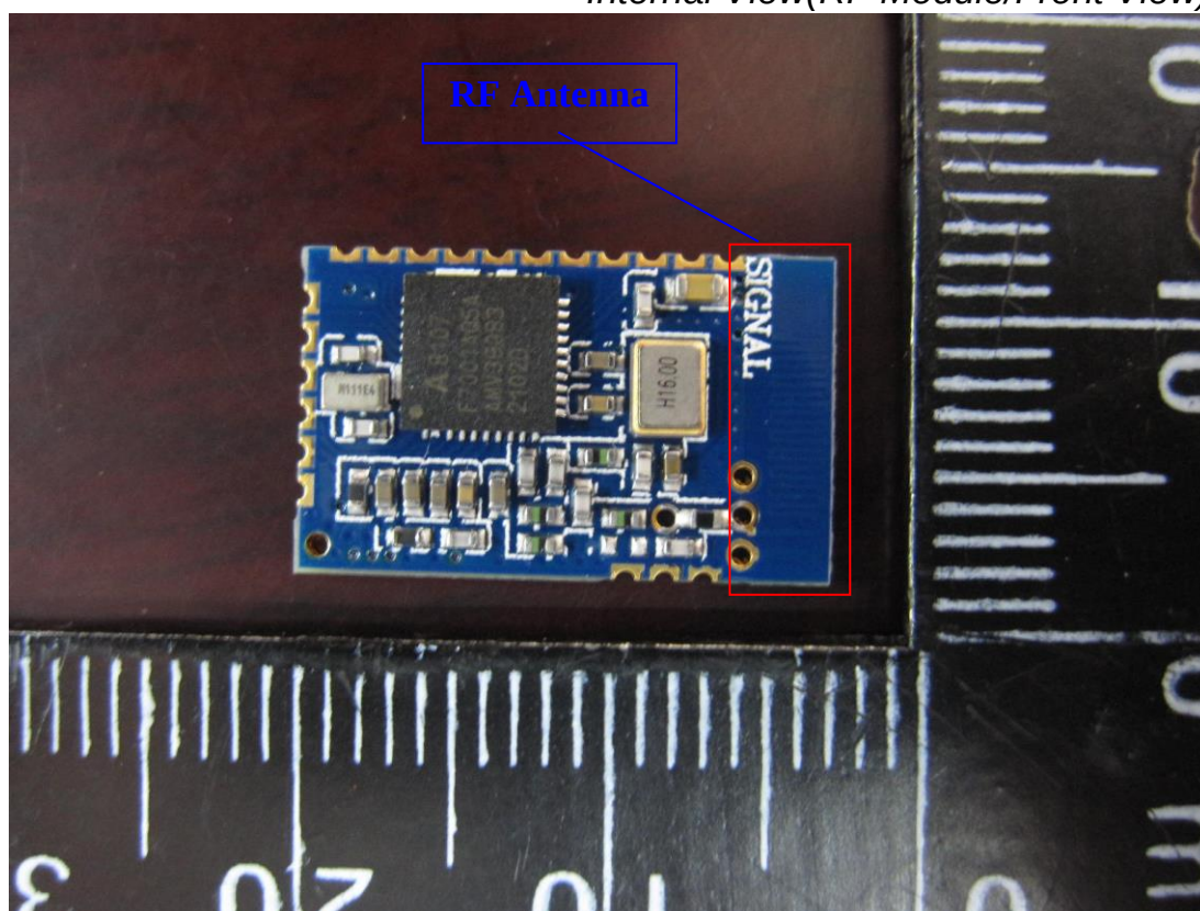
Figure 13 Internal View(RF Module/Front View)
