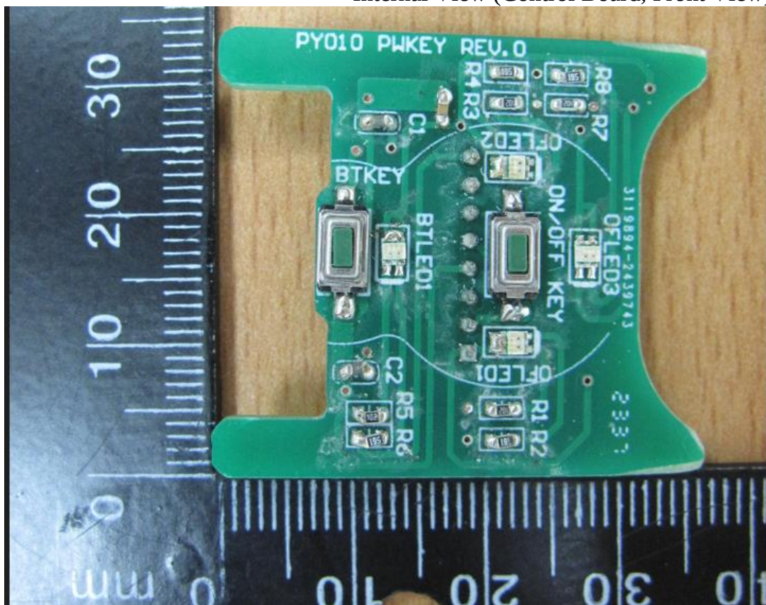
Figure 9 Internal View (Control Board, Front View)
