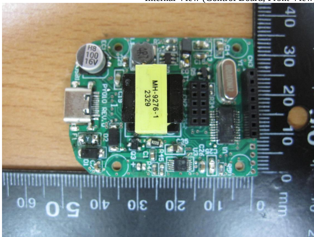
Figure 7 Internal View (Control Board, Front View)
