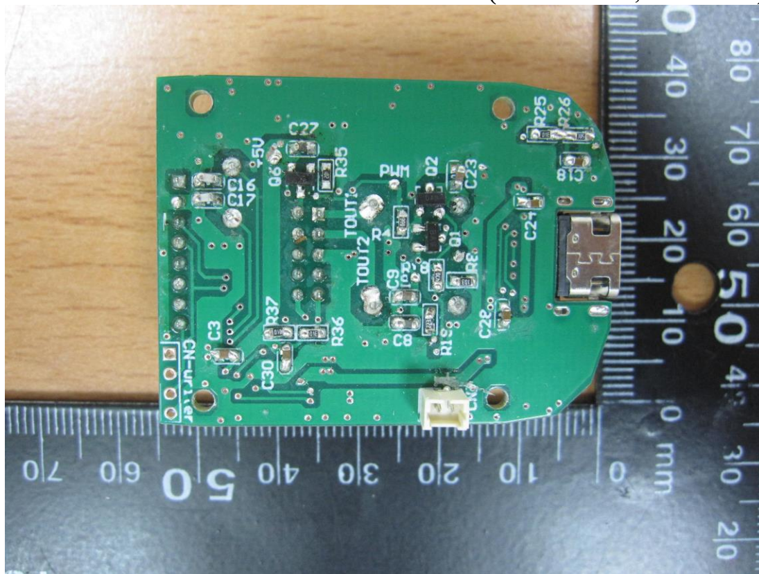
Figure 8 Internal View (Control Board, Front View)
