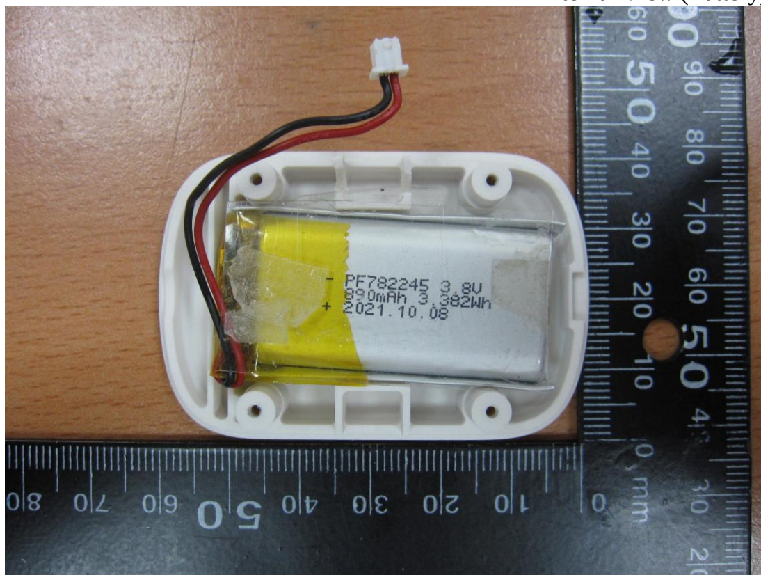
Figure 6 Internal View (Battery)
