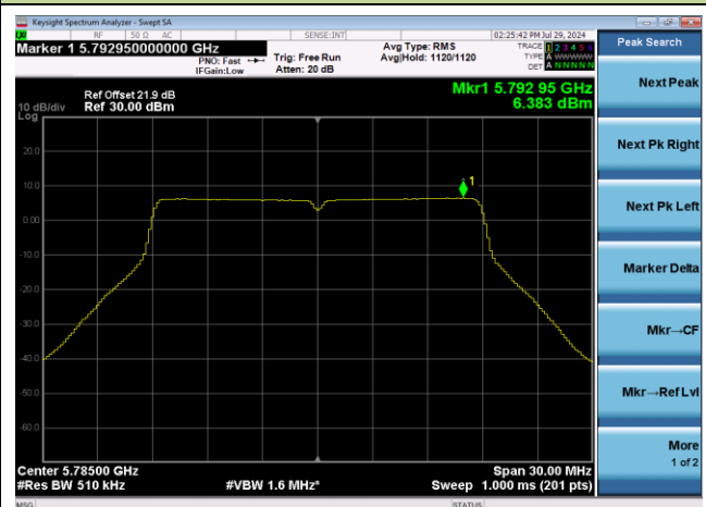
Channel 157 (5785MHz)
