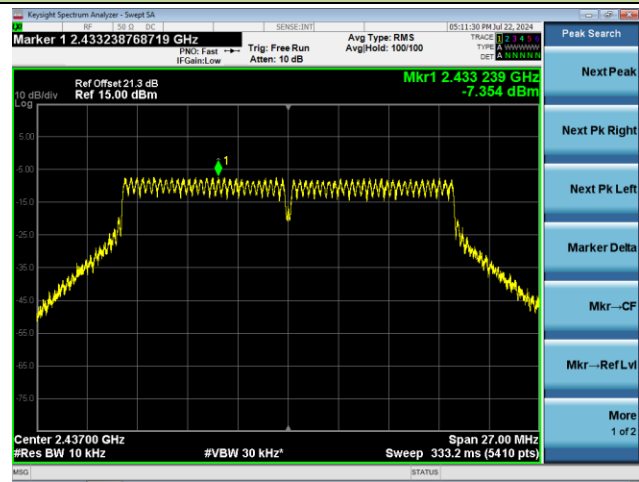
Channel 06 (2437MHz)
