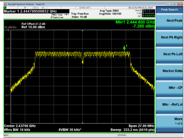
Channel 06 (2437MHz)
