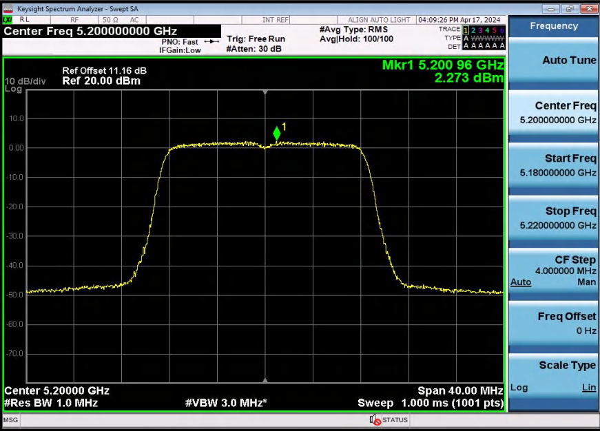
11A-Ant1-5200-PASS
