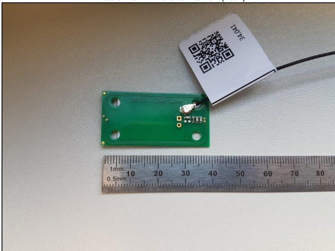
Photo 6: EUT - NFC antenna PCB (Back)
