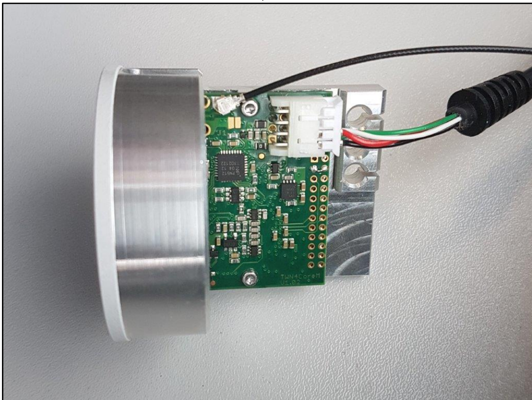
Photo 4: EUT - Side, Connectors and PCB
