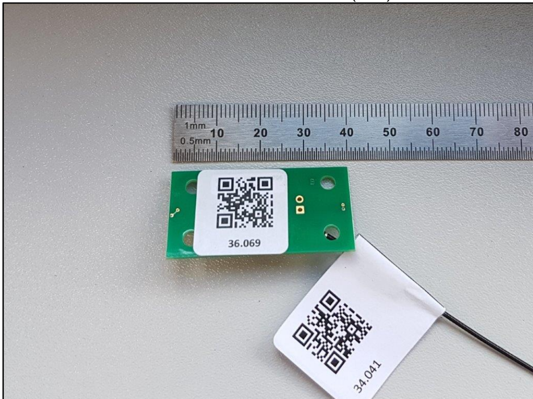
Photo 5: EUT - NFC antenna PCB (Front)
