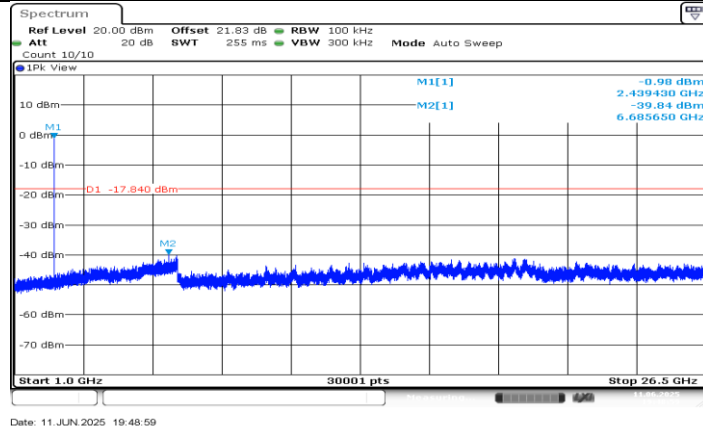
BLE_2M_Ant1_2440_1000~26500
