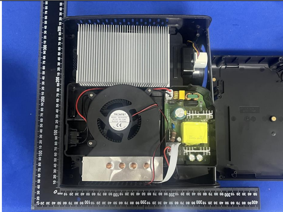
Internal photos
