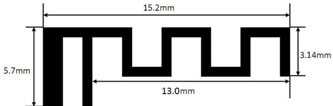
PCB Antenna Photo & Length (mm)
