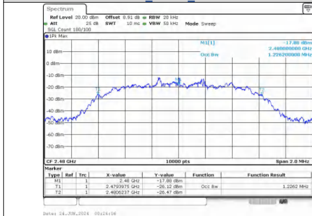
8DPSK_3-DH5_Channel 78
