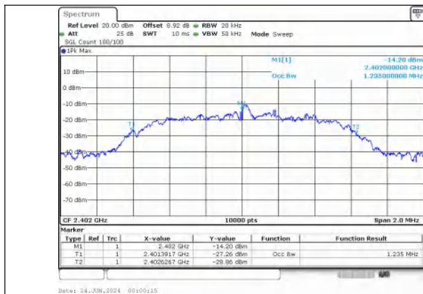
8DPSK_3-DH5_Channel 0
