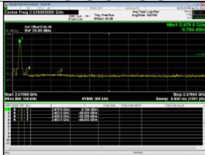
Pi/4DQPSK_2DH5_HCH_2480MHz_Ant1_NTNV
