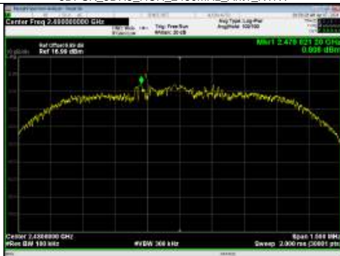
8DPSK_3DH5_HCH_2480MHz_Ant1_NTNV
