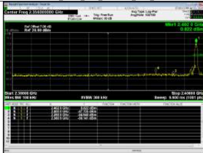
8DPSK_3DH5_LCH_2402MHz_Ant1_NTNV
