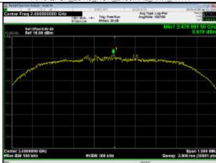
Pi/4DQPSK_2DH5_HCH_2480MHz_Ant1_NTNV
