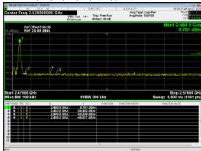
8DPSK_3DH5_HCH_2480MHz_Ant1_NTNV
