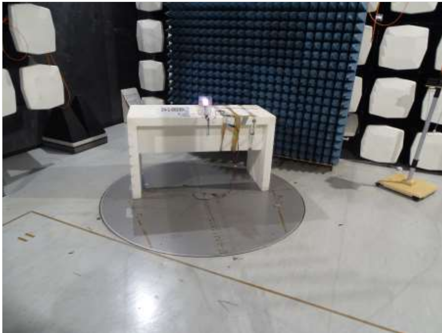
Photograph 3: EUT test setup in the semi- anechoic chamber
