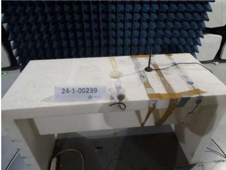
Photograph 1: EUT setup measurement, close up view
