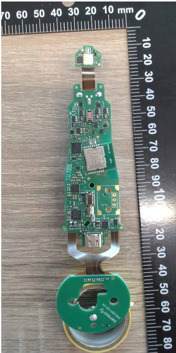
Figure 10: PCB front
