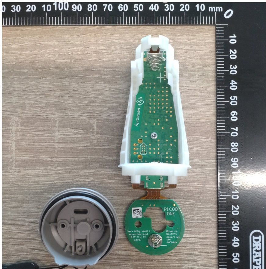
Figure 3: Inner frame back, battery and bottom cap removed
