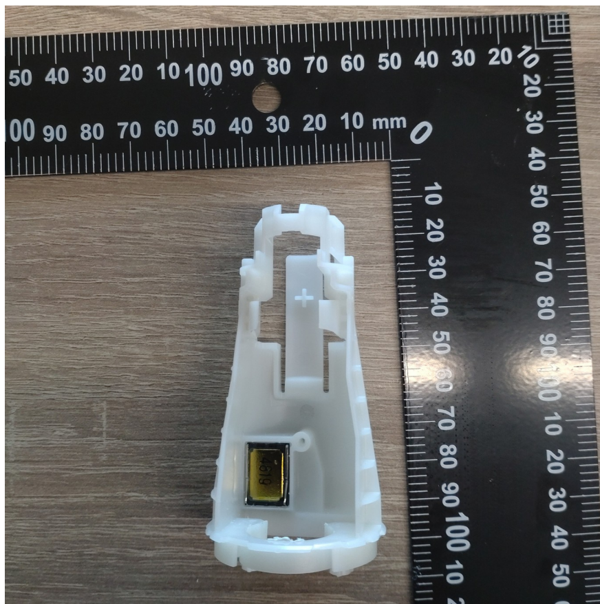
Figure 6: Inner frame back, PCB removed
