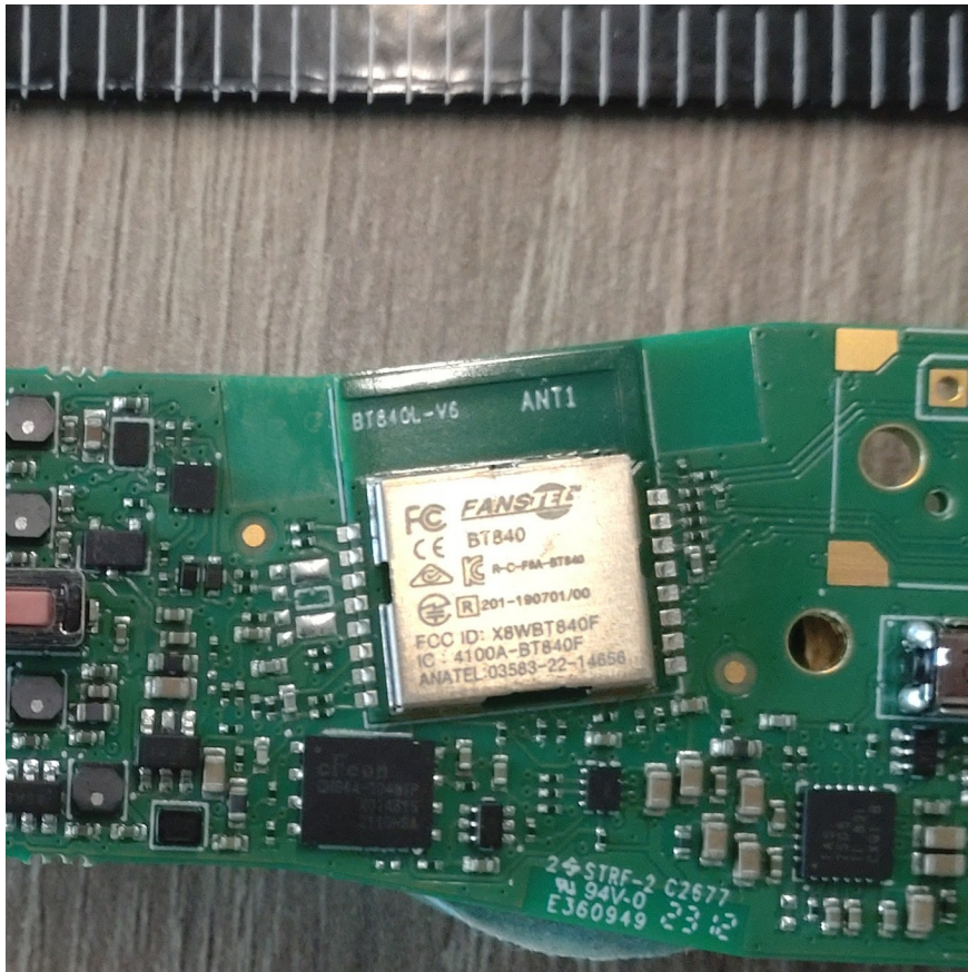
Figure 11: PCB front, BT840 module text
