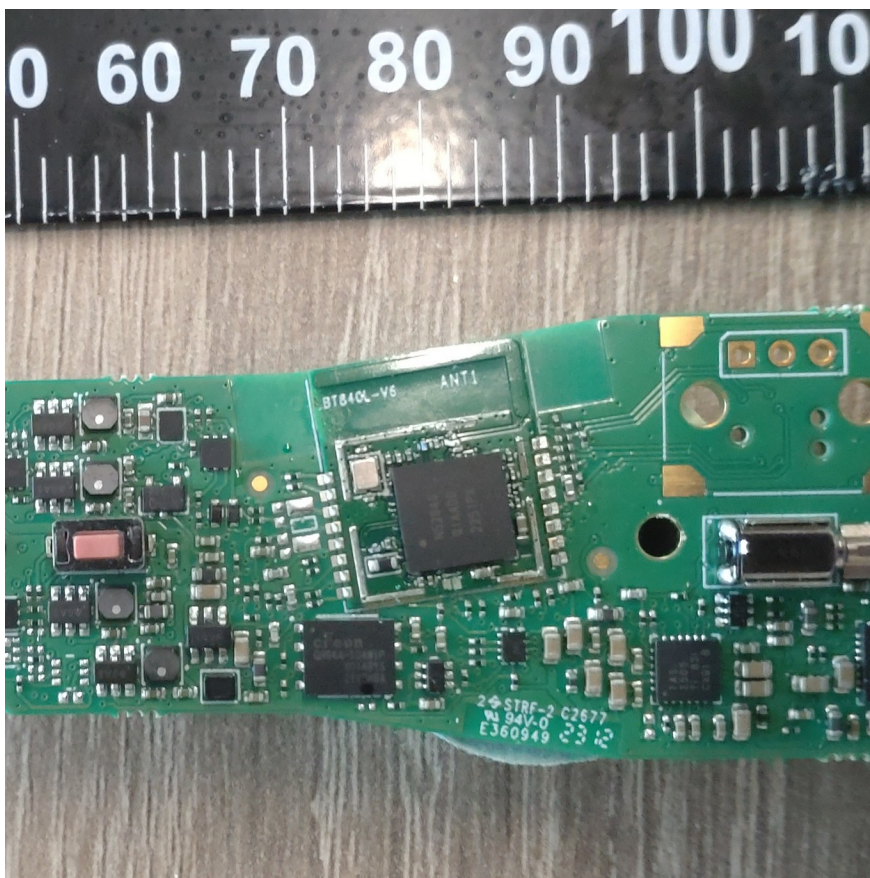
Figure 12: PCB front, BT840 shield removed
