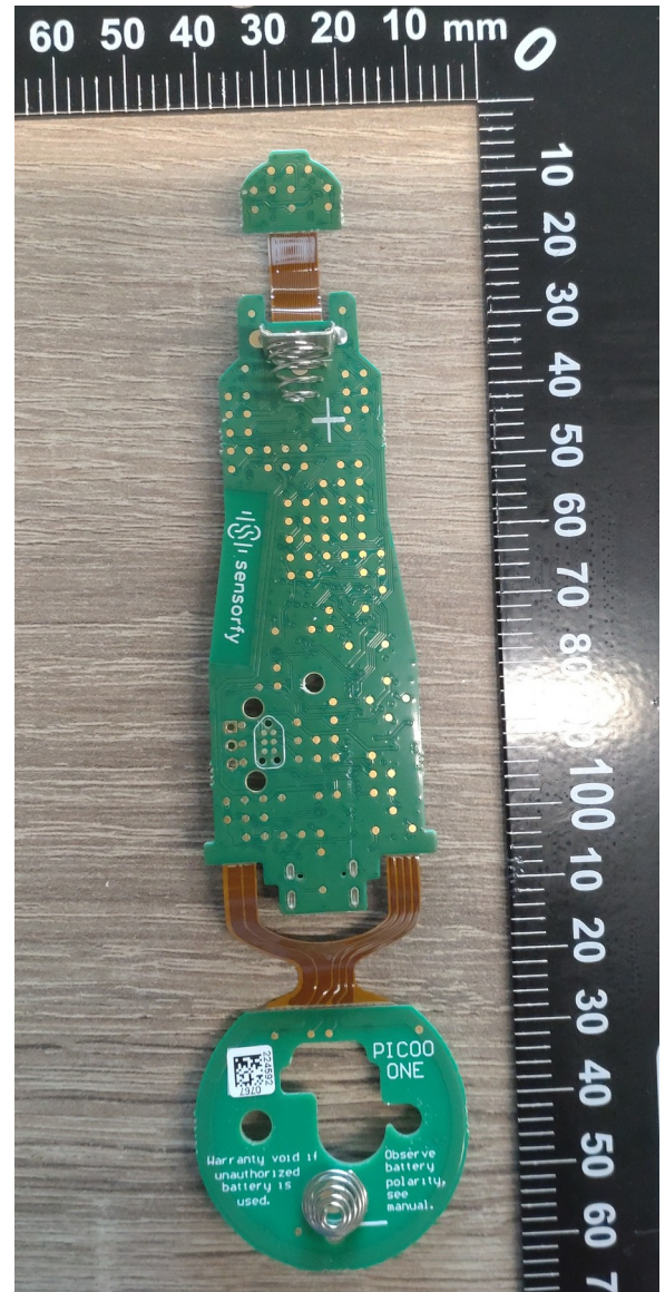
Figure 9: PCB back
