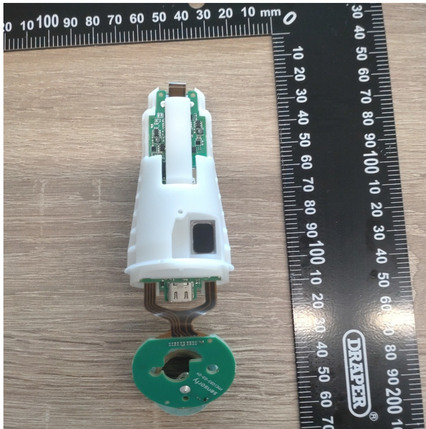
Figure 5: Inner frame front
