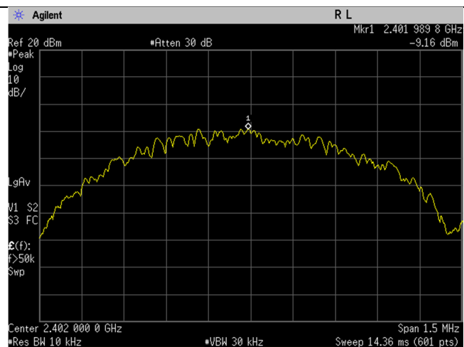
BLE_Low Ch_2402MHz_1MBit_Spectral Density
