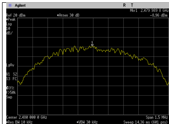
BLE_High Ch_2480MHz_1MBit_Spectral Density
