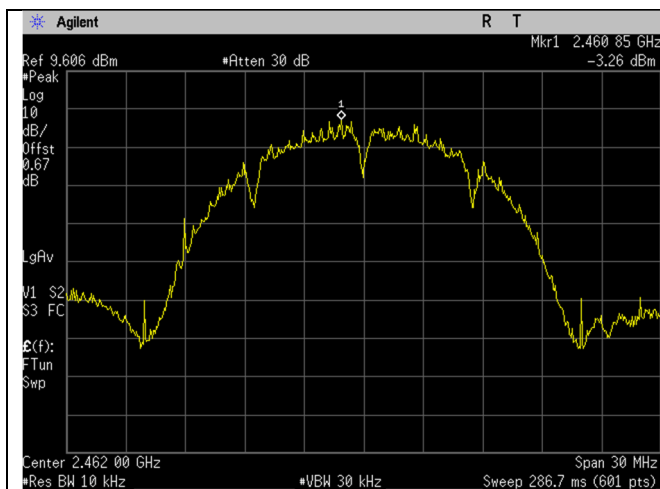
WIFI_High Ch_2462MHz_20MHz BW_b-mode_Spectral Density
