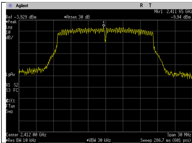
WIFI_Low Ch_2412MHz_20MHz BW_g-mode_Spectral Density
