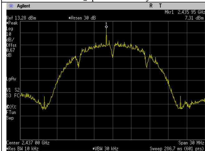
WIFI_Mid Ch_2437MHz_20MHz BW_b-mode_Spectral Density
