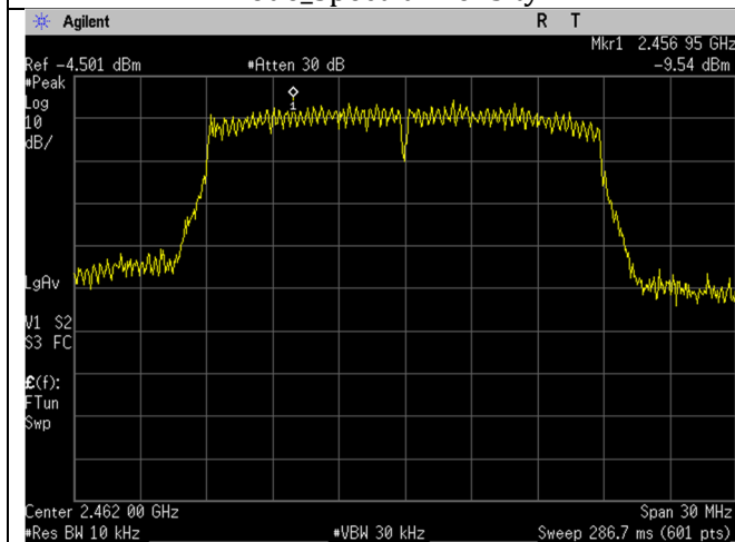
WIFI_High Ch_2462MHz_20MHz BW_n-mode_Spectral Density
