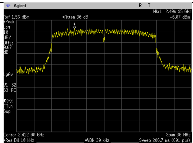
WIFI_Low Ch_2412MHz_20MHz BW_n-mode_Spectral Density
