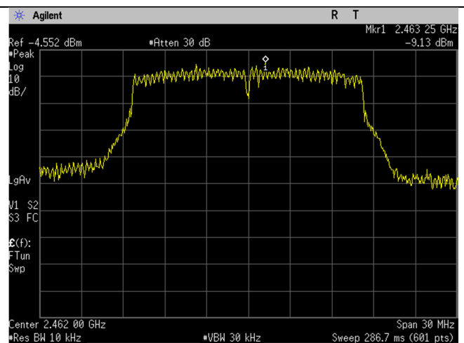
WIFI_High Ch_2462MHz_20MHz BW_g-mode_Spectral Density
