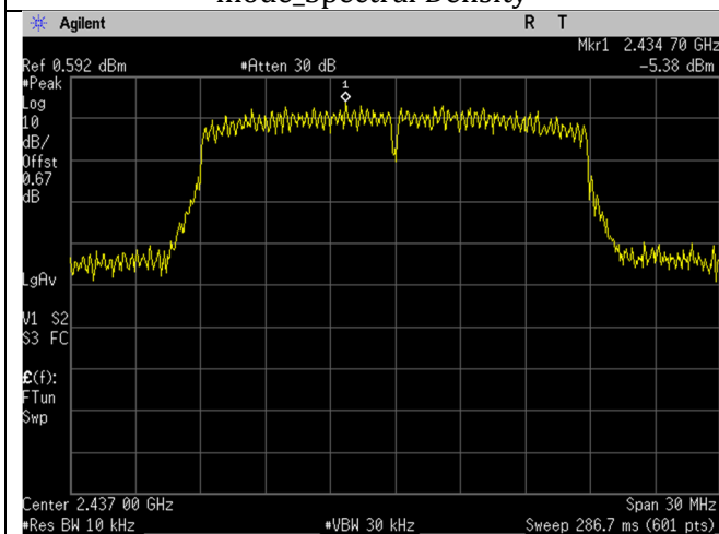
WIFI_Mid Ch_2437MHz_20MHz BW_n-mode_Spectral Density
