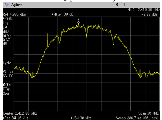
WIFI_Low Ch_2412MHz_20MHz BW_b-mode_Spectral Density
