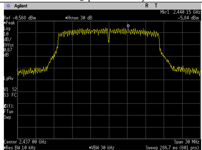
WIFI_Mid Ch_2437MHz_20MHz BW_g-mode_Spectral Density
