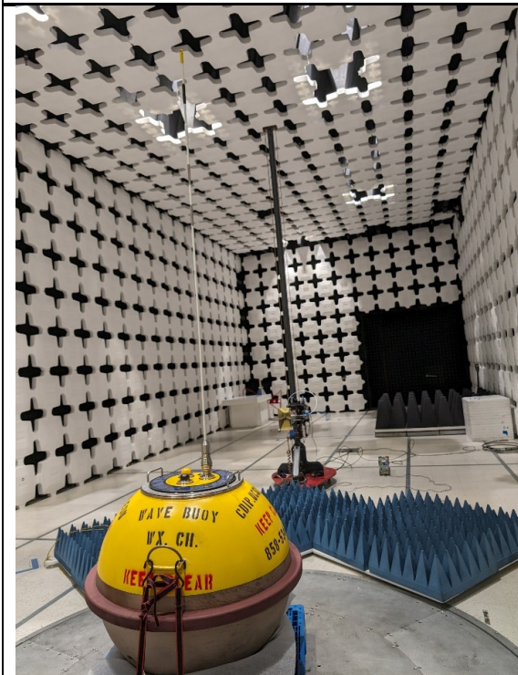
Radiated Emission-Above 1GHz-Front
