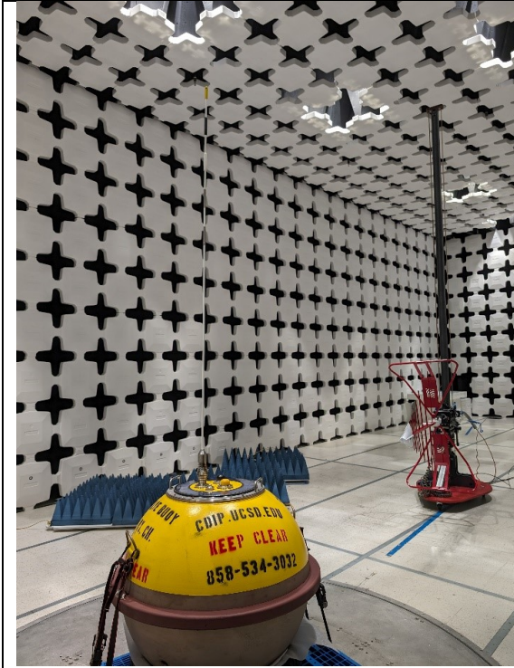
Radiated Emission-Below 1GHz-Front
