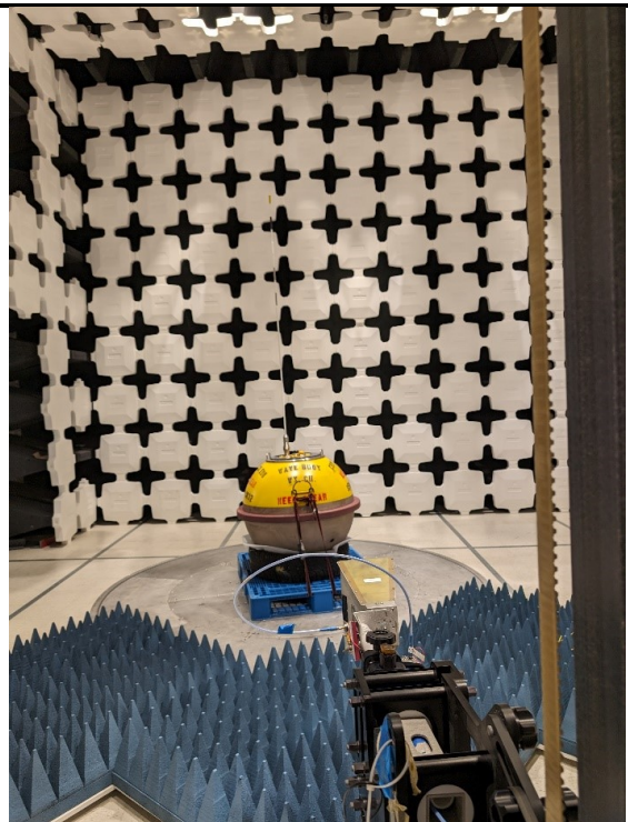
Radiated Emission-Above 1GHz-Back
