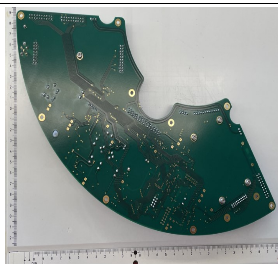
Main PCB Bottom View
