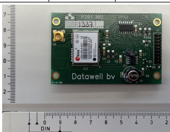
GPS Position PCB Top View
