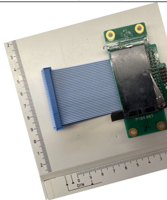
Compact Flash PCB Bottom View
