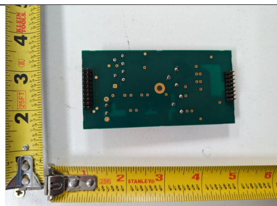
HF Transmitter PCB, 29.79 MHz, Rear View
