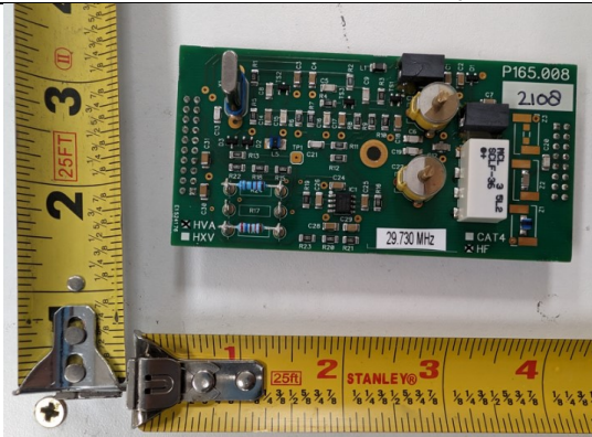
HF Transmitter PCB, 29.73 MHz, Front View
