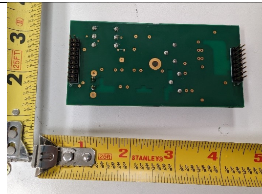
HF Transmitter PCB, 29.75 MHz, Rear View
