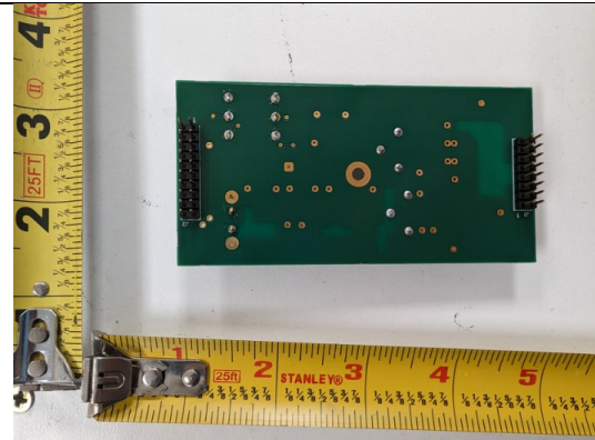
HF Transmitter PCB, 29.73 MHz, Rear View
