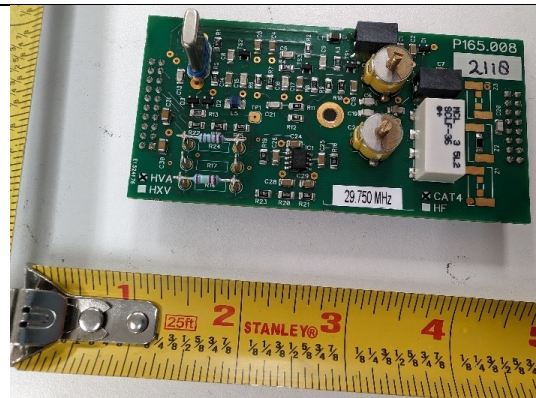
HF Transmitter PCB, 29.75 MHz, Front View
