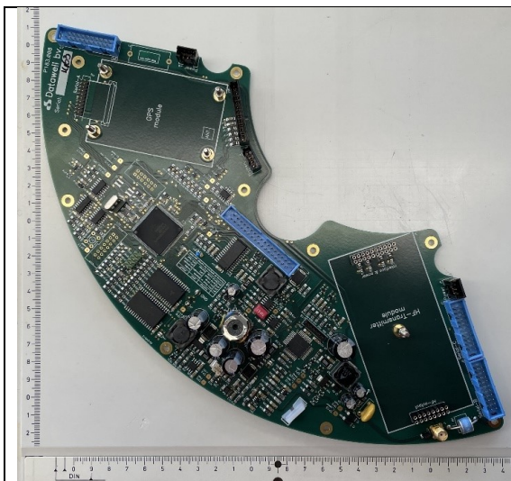
Main PCB Top View
