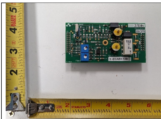
HF Transmitter PCB, 29.79 MHz, Front View
