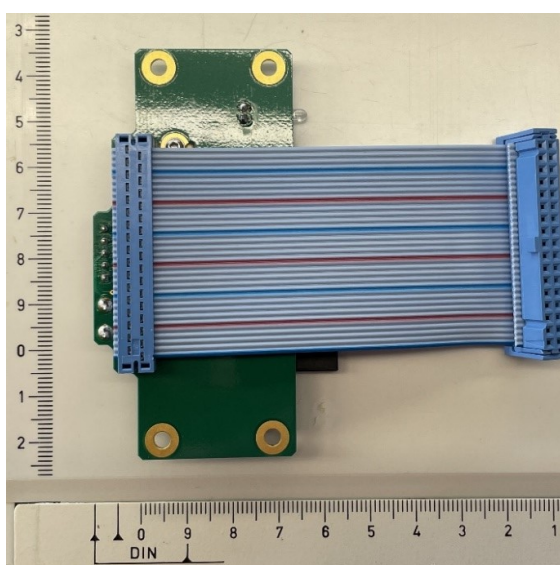
Compact Flash PCB Top View
