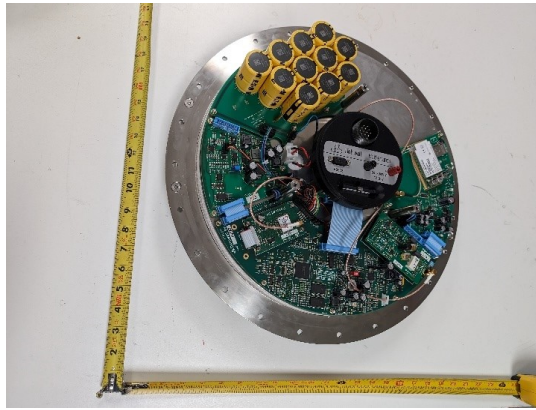
EUT, Hatch Cover, Internal Top View
