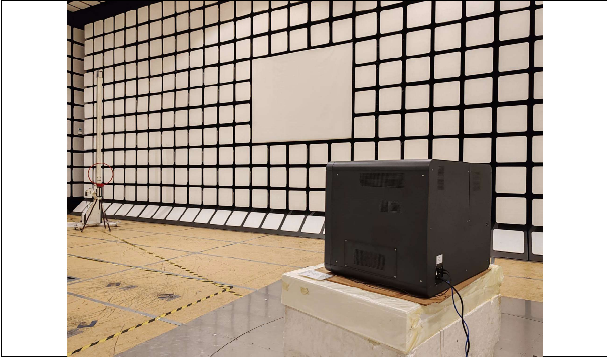
Radiated Emissions (Fundamental) Test Setup (Front View)
