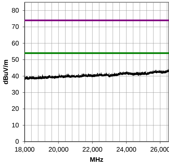
18000-26500 MHz, Run 8
