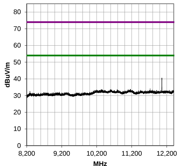
8200-12400 MHz, Run 6
