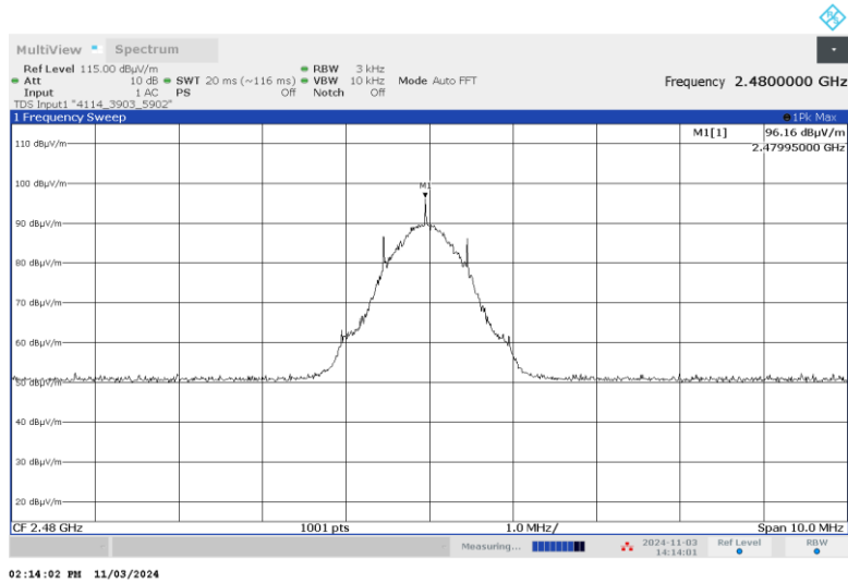
Plot 7.5.3 Peak spectral power density at high frequency (1 Mbps)
