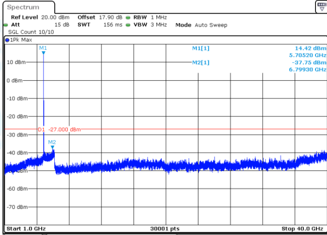
11AX20-CDD-Ant1-5700-1000~40000-PASS
