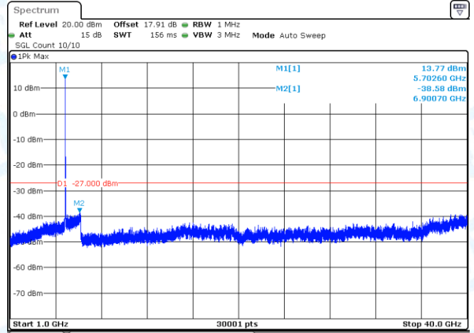
11AX20-CDD-Ant2-5700-1000~40000-PASS
