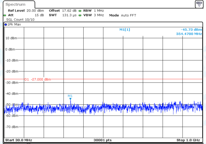
11AX80-CDD-Ant2-5530-30~1000-PASS
