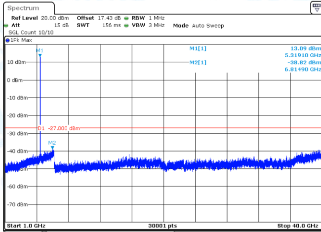
11AX20-CDD-Ant1-5320-1000~40000-PASS
