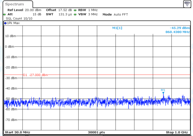
11AX20-CDD-Ant2-5280-30~1000-PASS
