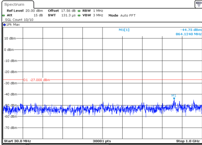
11AX80-CDD-Ant1-5530-30~1000-PASS
