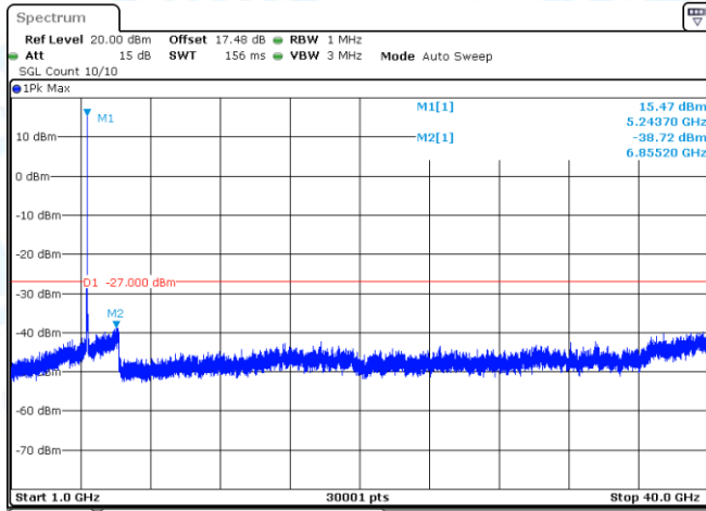
11AX20-CDD-Ant1-5240-1000~40000-PASS
