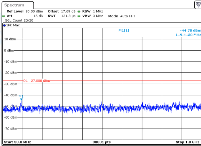
11AX40-CDD-Ant1-5795-30~1000-PASS
