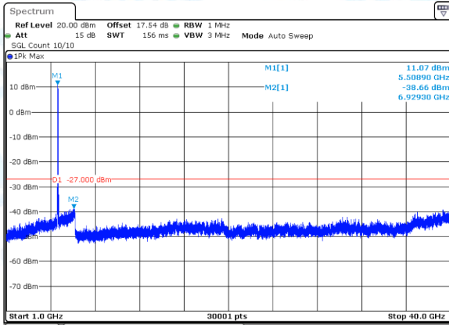
11AX40-CDD-Ant1-5510-1000~40000-PASS
