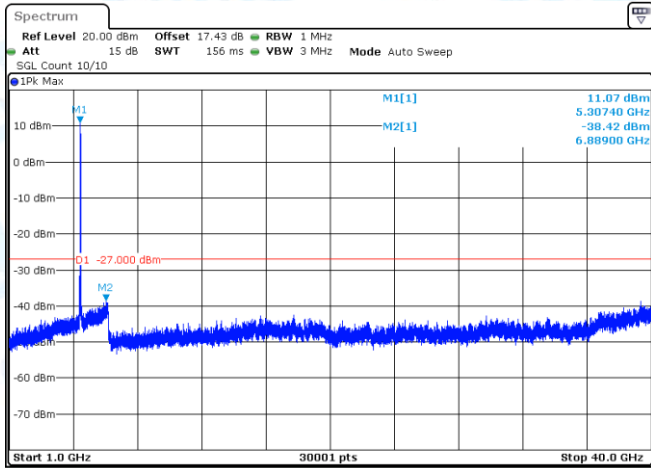
11AC40-CDD-Ant1-5310-1000~40000-PASS
