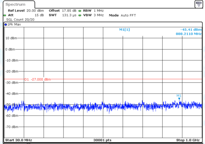
11AC20-CDD-Ant2-5825-30~1000-PASS
