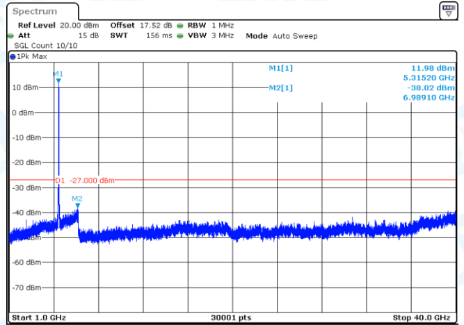
11AC40-CDD-Ant2-5310-1000~40000-PASS
