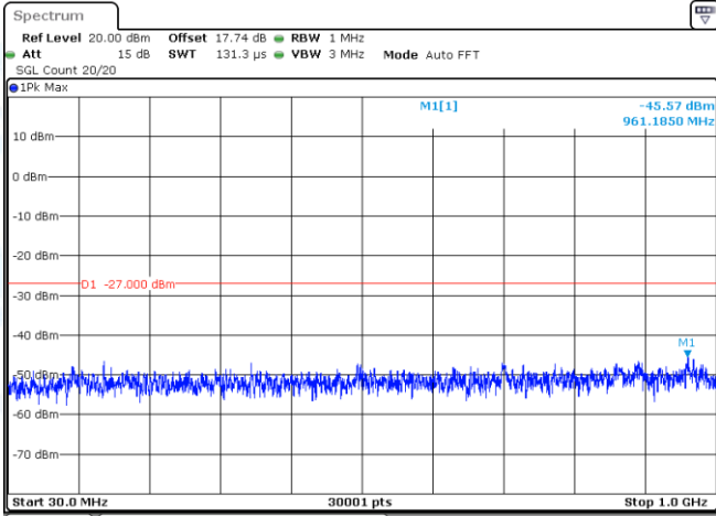
11AC20-CDD-Ant1-5825-30~1000-PASS
