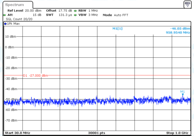
11AC40-CDD-Ant2-5755-30~1000-PASS
