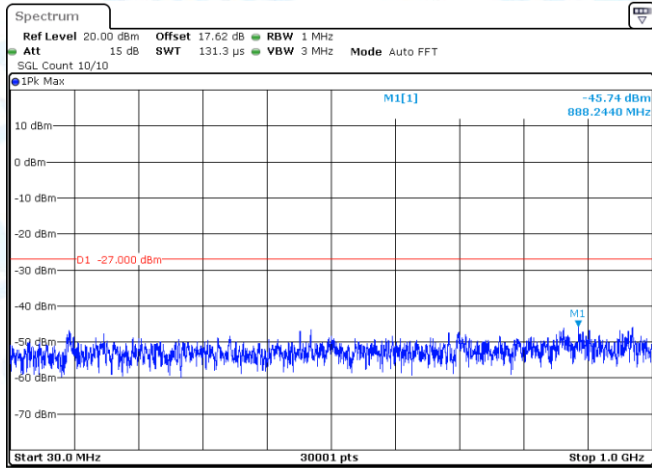
11AC40-CDD-Ant1-5550-30~1000-PASS
