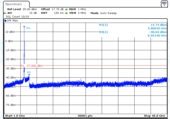
11AC40-CDD-Ant2-5795-1000~40000-PASS
