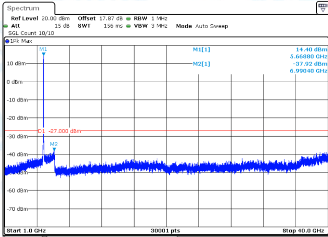
11AC40-CDD-Ant1-5670-1000~40000-PASS
