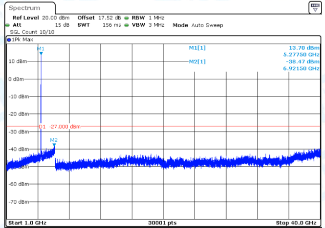
11AC20-CDD-Ant2-5280-1000~40000-PASS
