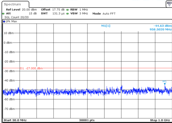
11AC40-CDD-Ant1-5755-30~1000-PASS
