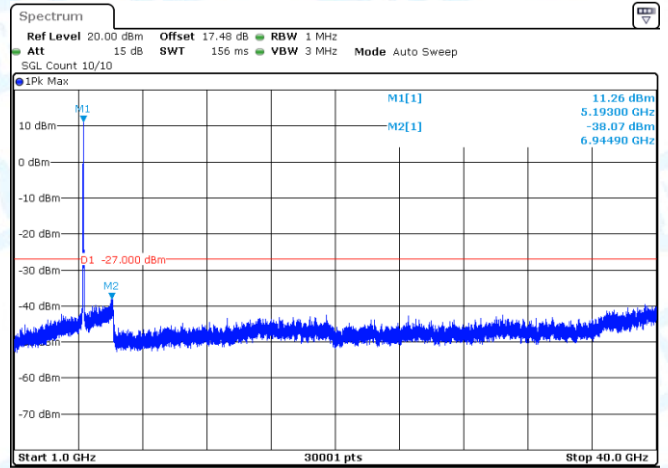
11AC40-CDD-Ant2-5190-1000~40000-PASS
