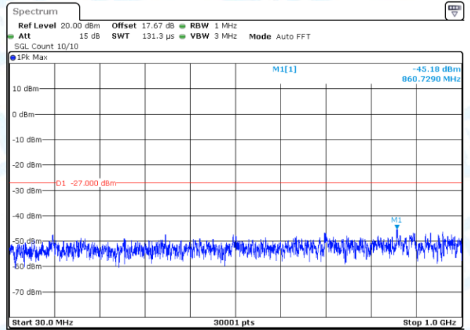
11AC40-CDD-Ant2-5550-30~1000-PASS
