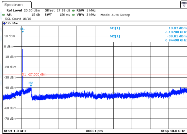
11AC40-CDD-Ant1-5190-1000~40000-PASS
