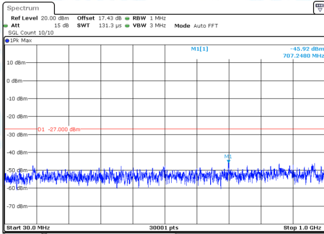
11AC80-CDD-Ant1-5290-30~1000-PASS
