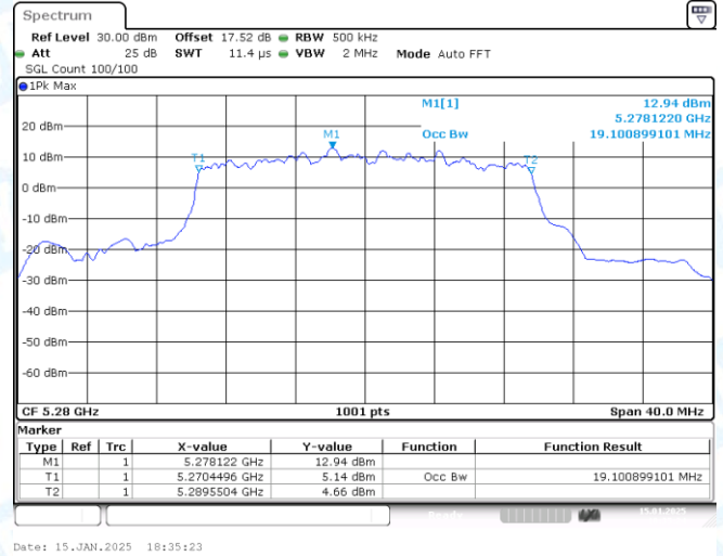
11AX20-CDD-Ant2-5280
