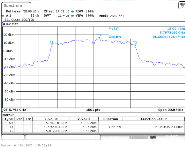
11N40-CDD-Ant1-5795
