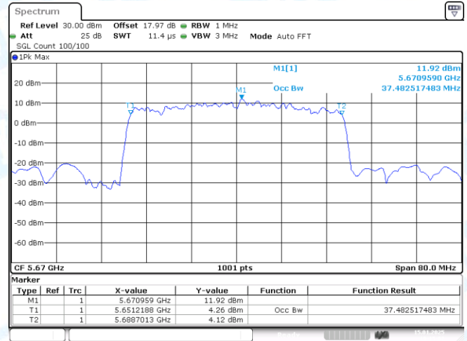
11AX40-CDD-Ant2-5670
