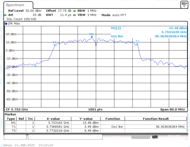
11N40-CDD-Ant2-5755
