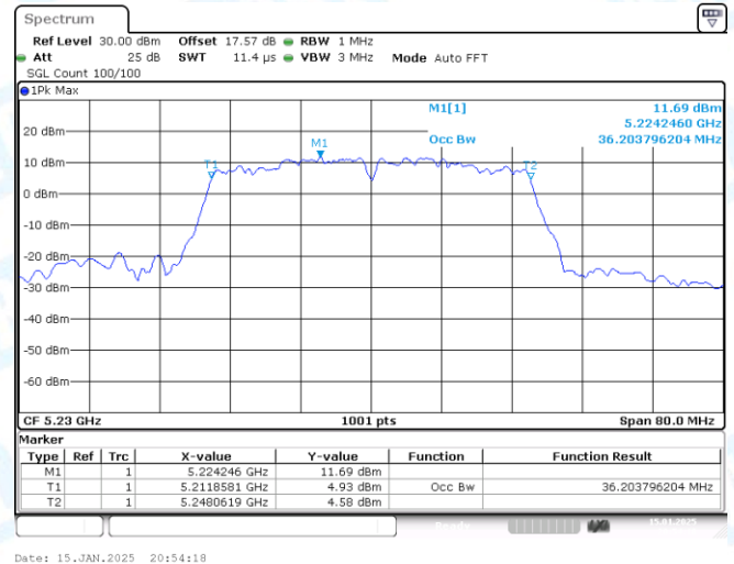
11AC40-CDD-Ant2-5230
