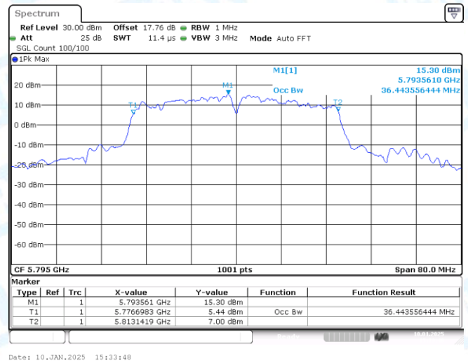
11N40-CDD-Ant2-5795
