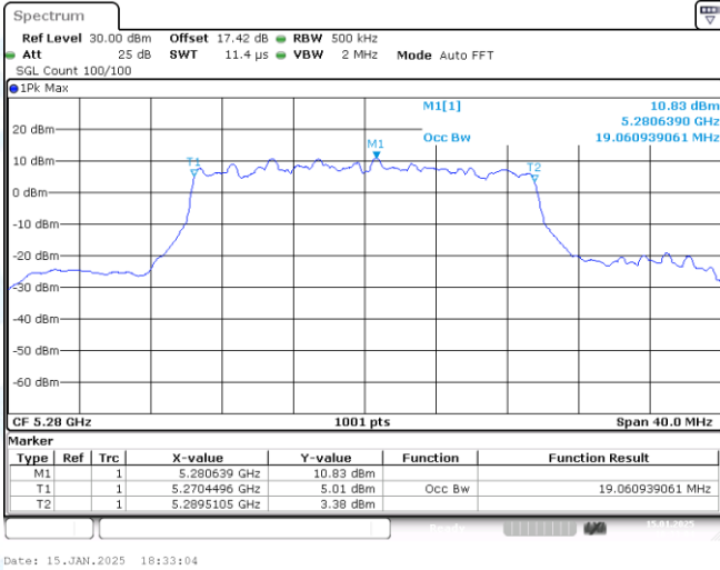
11AX20-CDD-Ant1-5280
