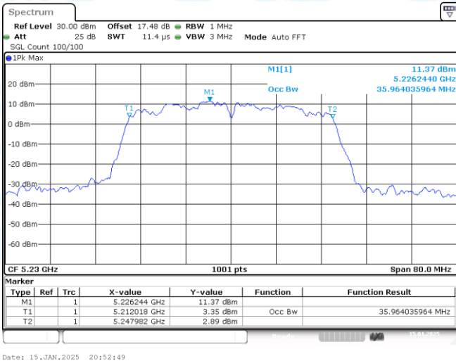
11AC40-CDD-Ant1-5230
