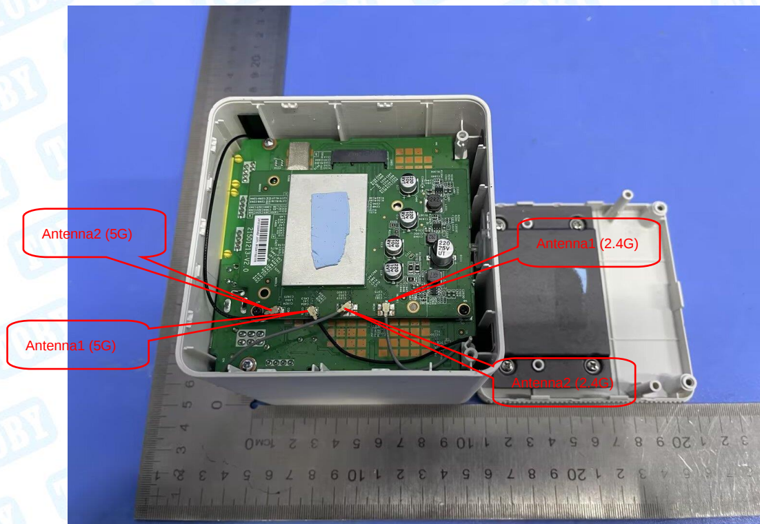
Photo 10 Internal of EUT
