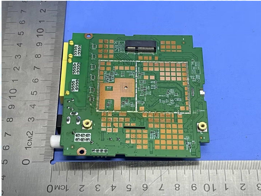
Photo 17 Appearance of PCB
