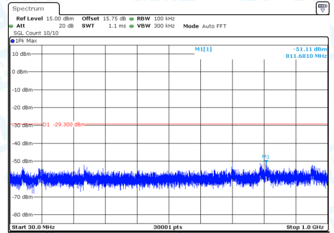
11N40-CDD-Ant2-2422-0~Reference-PASS
