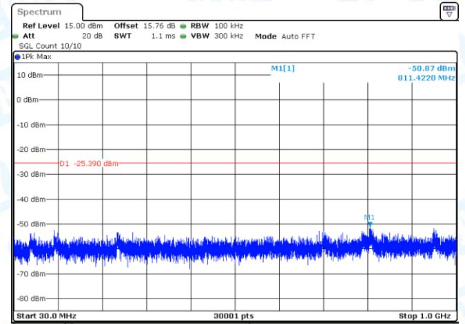
11N20-CDD-Ant2-2412-0~Reference-PASS
