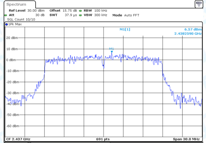
11N20-CDD-Ant2-2437-0~Reference-PASS
