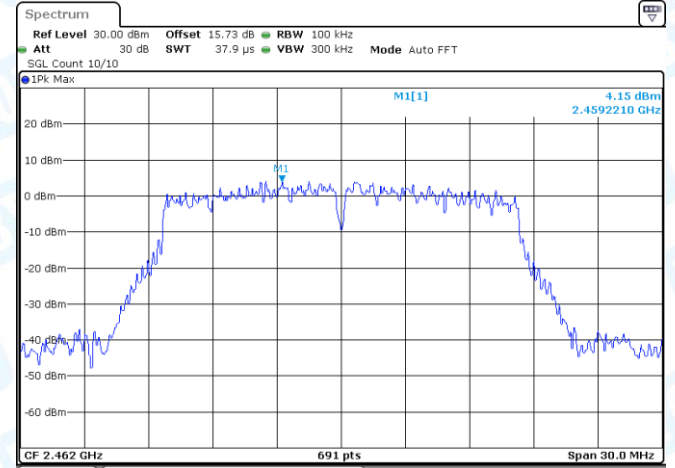
11G-Ant2-2462-0~Reference-PASS
