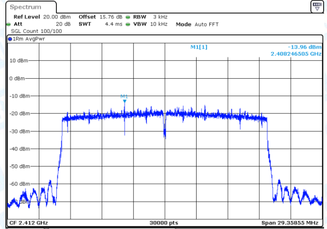
11AX20-CDD-Ant2-2412-PASS
