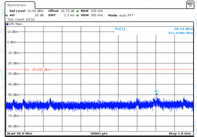
11G-Ant2-2462-0~Reference-PASS
