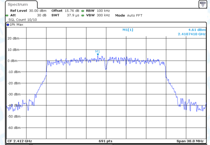
11N20-CDD-Ant2-2412-0~Reference-PASS
