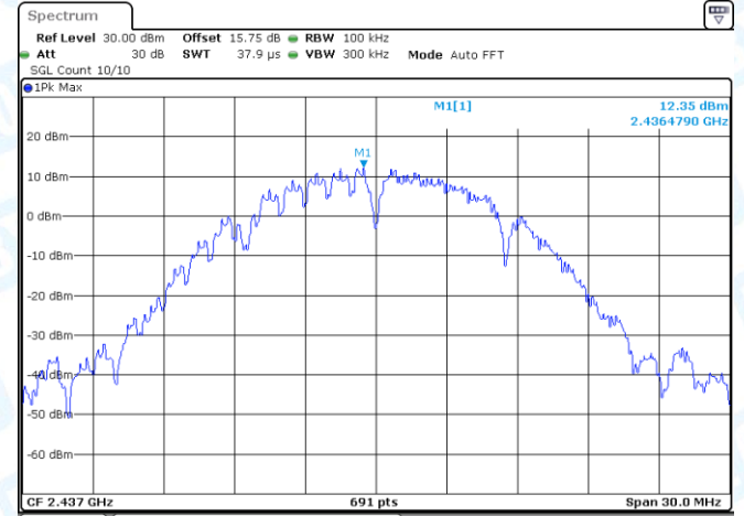
11B-Ant2-2437-0~Reference-PASS
