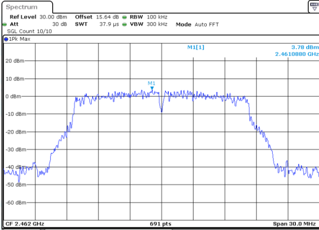
11G-Ant1-2462-0~Reference-PASS
