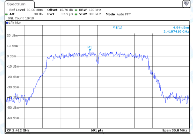
11G-Ant2-2412-0~Reference-PASS
