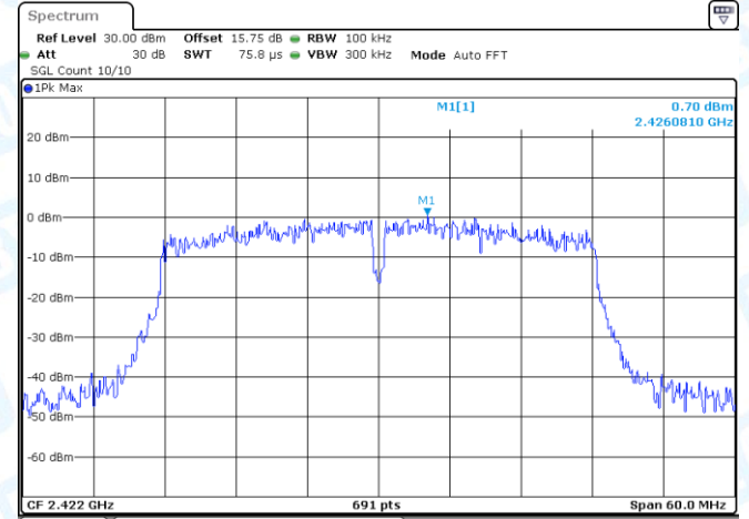
11N40-CDD-Ant2-2422-0~Reference-PASS
