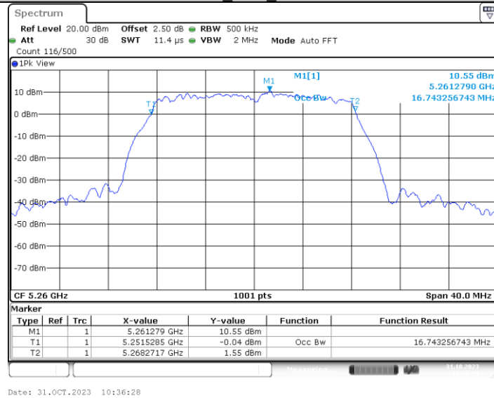
11A_Ant4_5260
