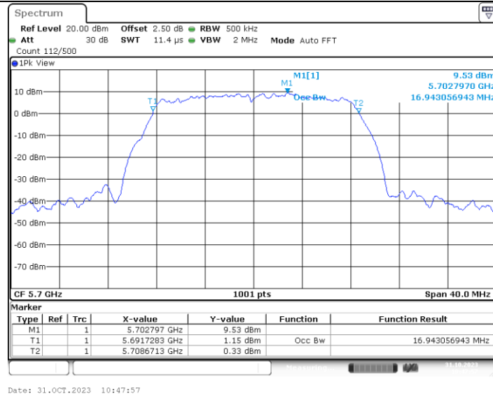
11A_Ant4_5700
