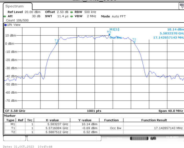
11A_Ant4_5580
