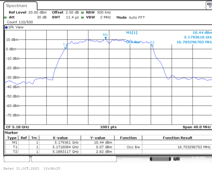
11A_Ant3_5180
