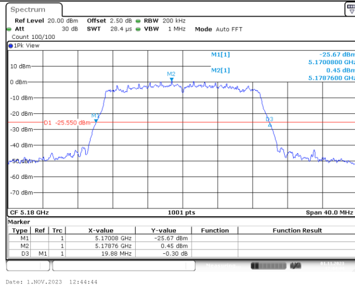
11AC20MIMO_Ant4_5180
