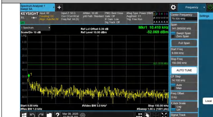
Band71-15MHz-QPSK-133297-1RB#0-0.009~0.15-PASS
