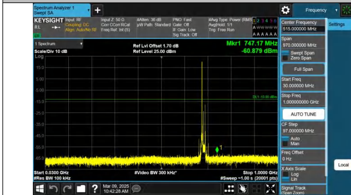
Band71-15MHz-QPSK-133397-1RB#0-30~1000-PASS
