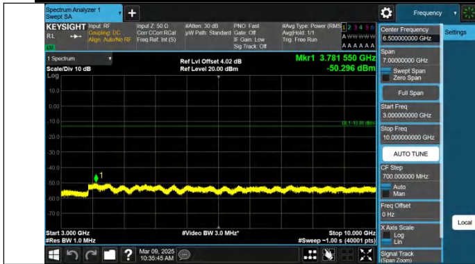
Band71-15MHz-QPSK-133197-1RB#0-3000~10000-PASS
