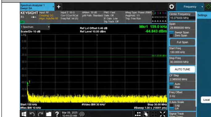
Band71-15MHz-QPSK-133397-1RB#74-0.15~30-PASS
