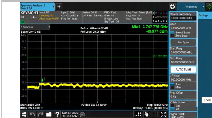
Band71-15MHz-QPSK-133397-1RB#0-3000~10000-PASS
