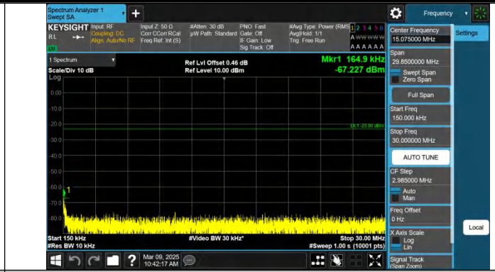
Band71-15MHz-QPSK-133397-1RB#0-0.15~30-PASS
