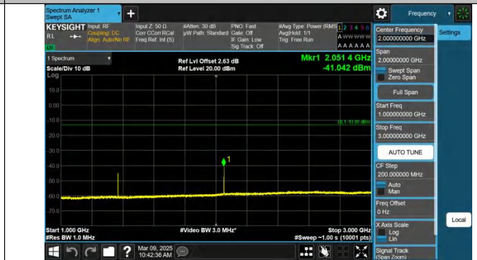
Band71-15MHz-QPSK-133397-1RB#0-1000~3000-PASS
