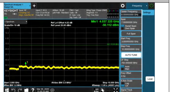
Band71-20MHz-QPSK-133372-1RB#99-3000~10000-PASS
