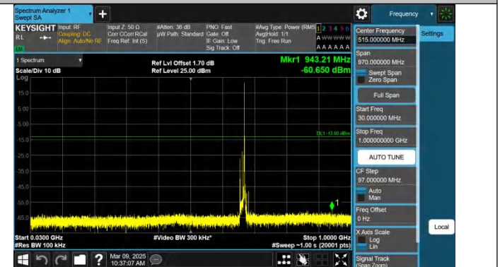
Band71-15MHz-QPSK-133197-1RB#74-30~1000-PASS
