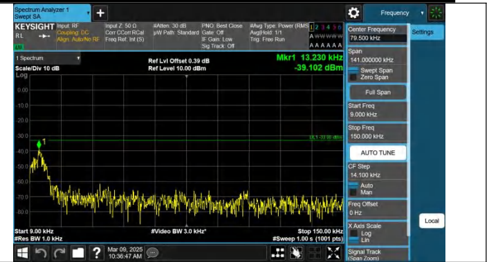
Band71-15MHz-QPSK-133197-1RB#74-0.009~0.15-PASS
