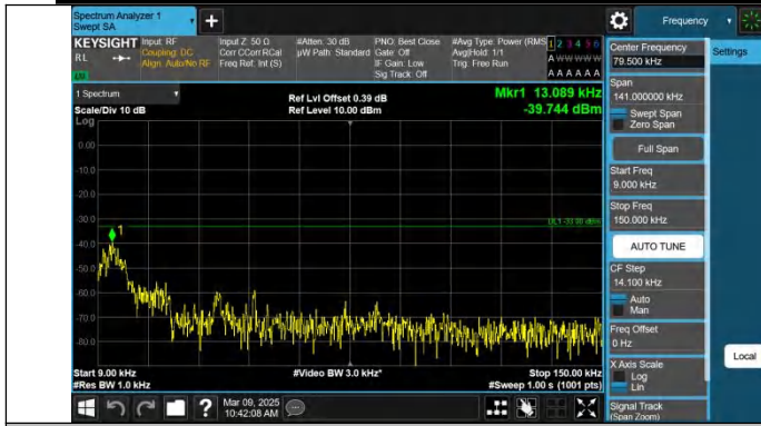
Band71-15MHz-QPSK-133397-1RB#0-0.009~0.15-PASS
