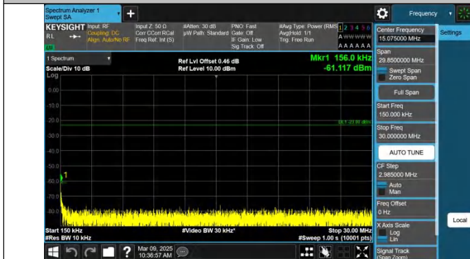
Band71-15MHz-QPSK-133197-1RB#74-0.15~30-PASS
