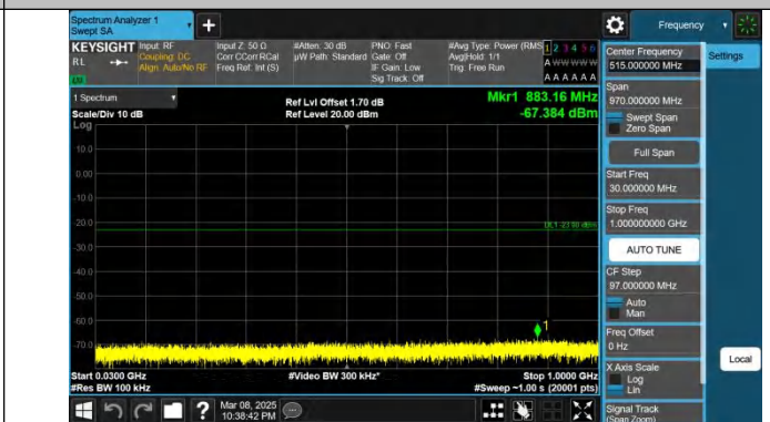
Band66-1.4MHz-QPSK-132665-1RB#5-30~1000-PASS
