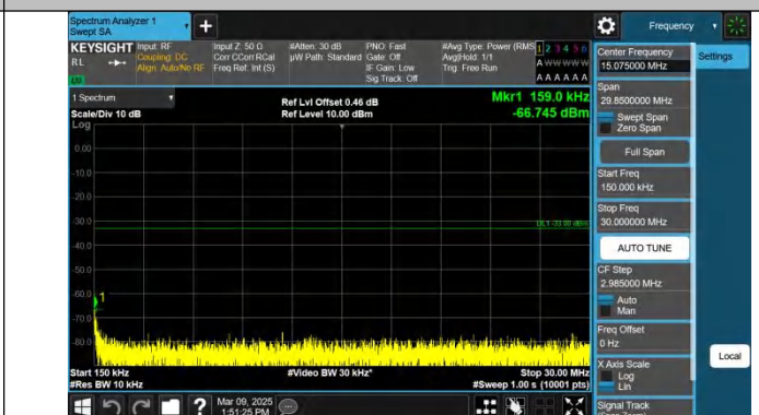
Band66-3MHz-QPSK-131987-1RB#0-0.15~30-PASS
