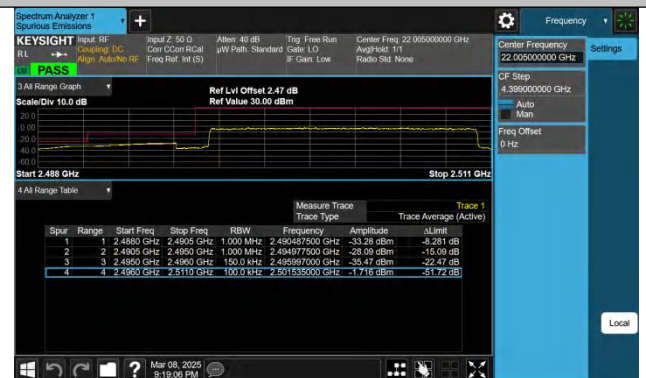
Band41-15MHz-QPSK-39725-75RB#0-PASS
