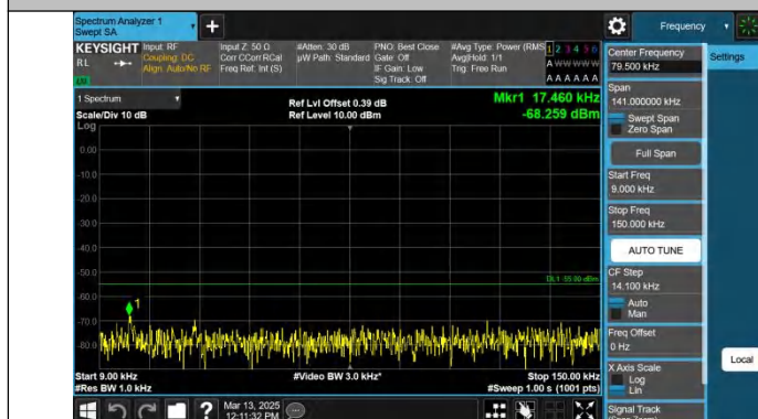
Band41-10MHz-QPSK-39700-1RB#0-0.009~0.15-PASS
