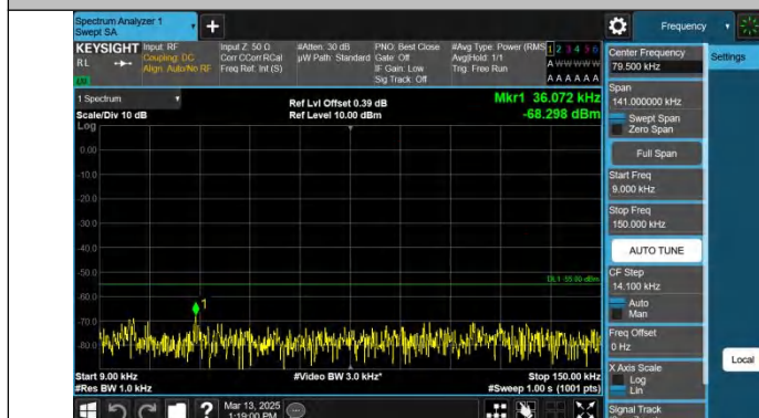
Band41-5MHz-QPSK-41565-1RB#0-0.009~0.15-PASS
