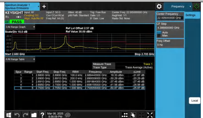
Band41-10MHz-QPSK-41540-1RB#49-PASS
