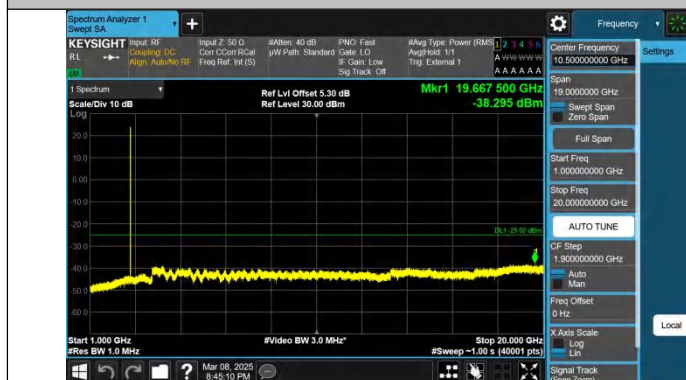
Band41-5MHz-QPSK-41565-1RB#24-1000~20000-PASS
