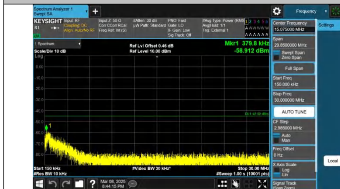
Band41-5MHz-QPSK-41565-1RB#24-0.15~30-PASS
