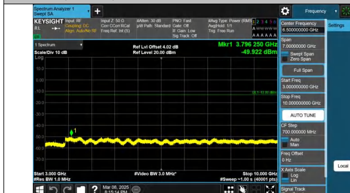
Band26(824-849)-15MHz-QPSK-26865-1RB#0-3000~10000-PAS
