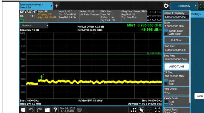
Band26(824-849)-15MHz-QPSK-26965-1RB#0-3000~10000-PASS S
