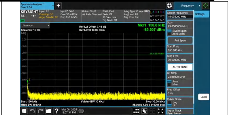
Band26(824-849)-10MHz-QPSK-26990-1RB#0-0.15~30-PASS
