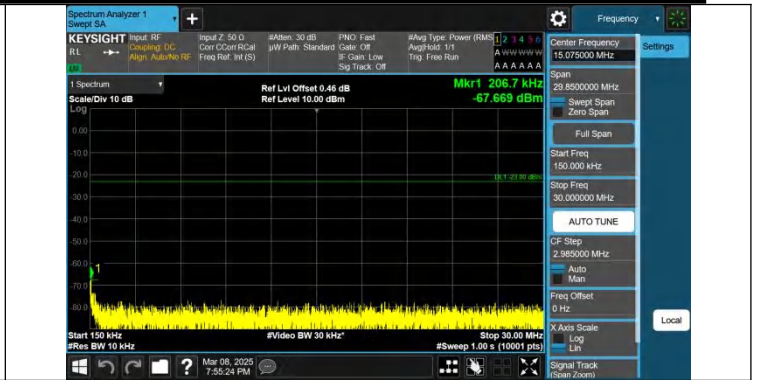
Band26(824-849)-5MHz-QPSK-26915-1RB#0-0.15~30-PASS
