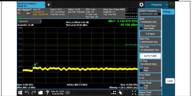
Band26(824-849)-10MHz-QPSK-26990-1RB#49-3000~10000-PAS
