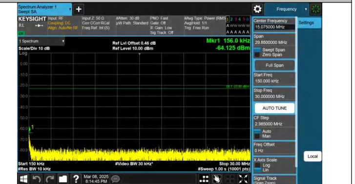
Band26(824-849)-15MHz-QPSK-26865-1RB#0-0.15~30-PASS
