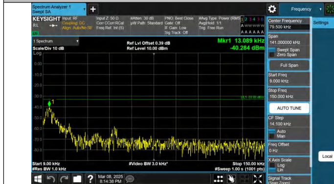
Band26(824-849)-15MHz-QPSK-26865-1RB#0-0.009~0.15-PASS
