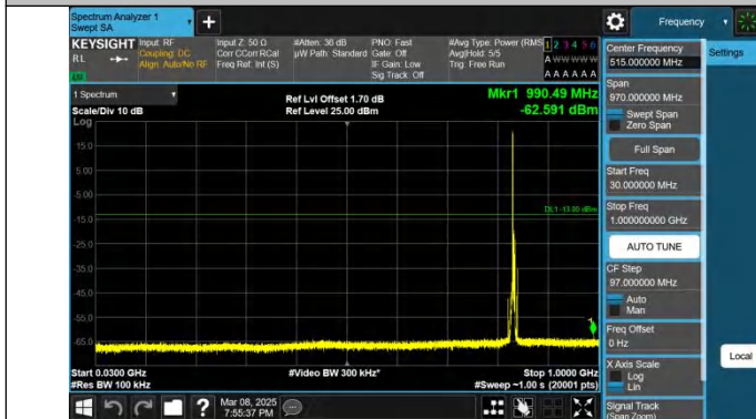
Band26(824-849)-5MHz-QPSK-26915-1RB#0-30~1000-PASS
