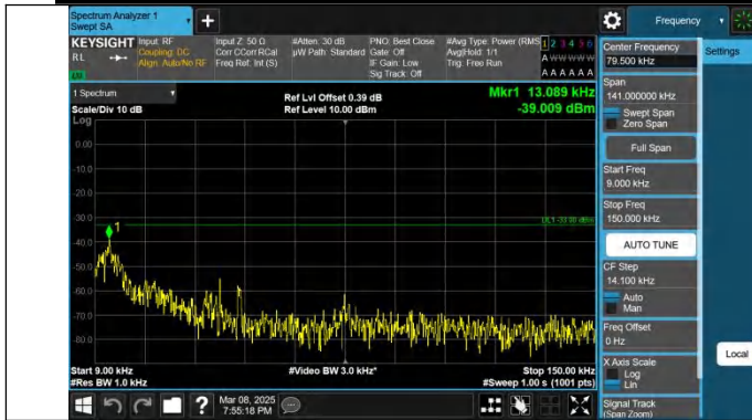
Band26(824-849)-5MHz-QPSK-26915-1RB#0-0.009~0.15-PASS
