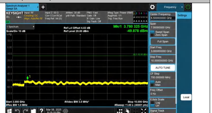
Band26(824-849)-15MHz-QPSK-26965-1RB#74-3000~10000-PASS S
