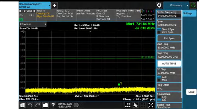
Band25-15MHz-QPSK-26365-1RB#74-30~1000-PASS
