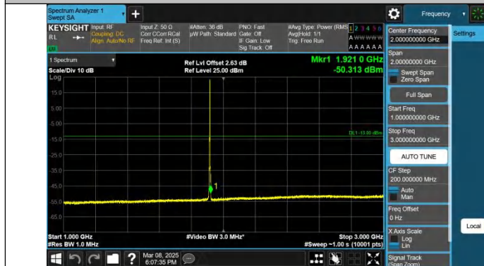
Band25-3MHz-QPSK-26675-1RB#14-1000~3000-PASS
