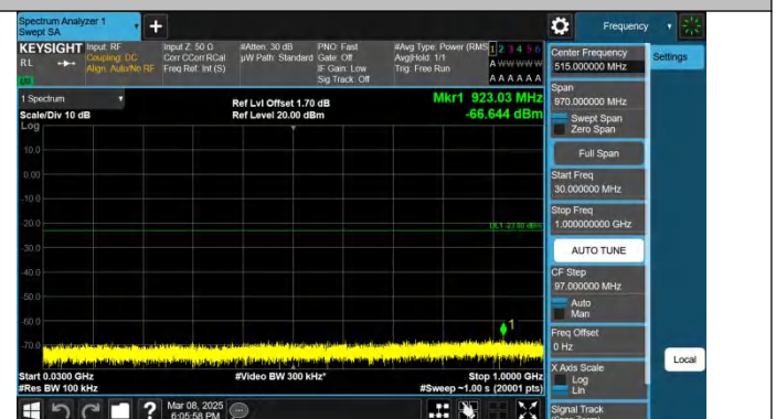
Band25-3MHz-QPSK-26365-1RB#14-30~1000-PASS
