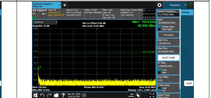
Band25-20MHz-QPSK-26590-1RB#0-0.15~30-PASS
