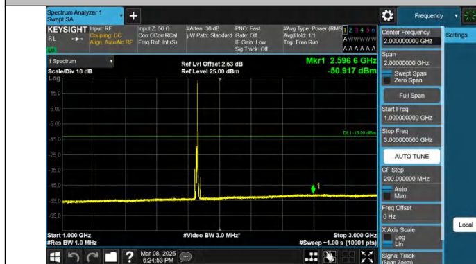
Band25-10MHz-QPSK-26090-1RB#49-1000~3000-PASS
