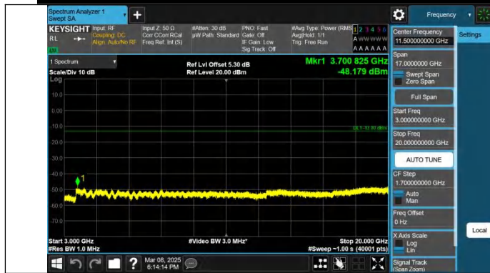
Band25-5MHz-QPSK-26065-1RB#0-3000~20000-PASS
