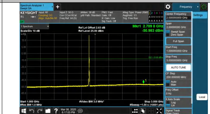
Band25-5MHz-QPSK-26665-1RB#0-1000~3000-PASS
