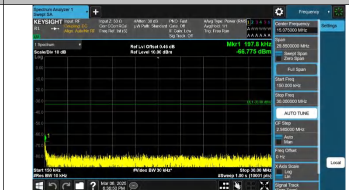
Band25-15MHz-QPSK-26615-1RB#0-0.15~30-PASS
