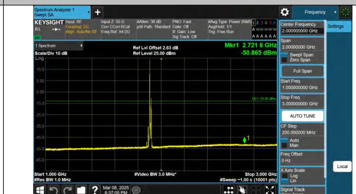
Band25-15MHz-QPSK-26615-1RB#0-1000~3000-PASS
