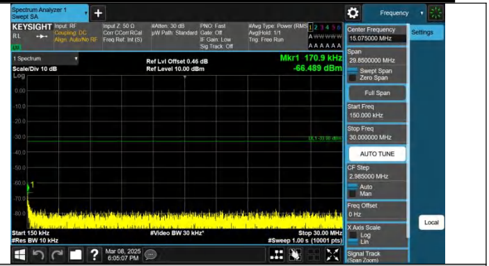
Band25-3MHz-QPSK-26365-1RB#0-0.15~30-PASS
