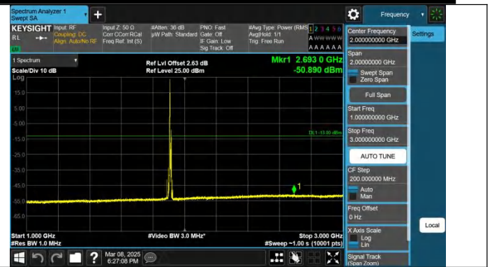
Band25-10MHz-QPSK-26640-1RB#0-1000~3000-PASS
