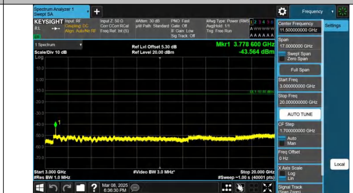
Band25-15MHz-QPSK-26365-1RB#74-3000~20000-PASS
