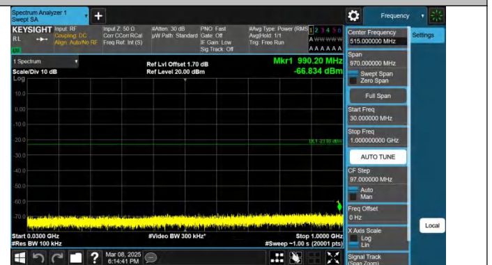
Band25-5MHz-QPSK-26065-1RB#24-30~1000-PASS
