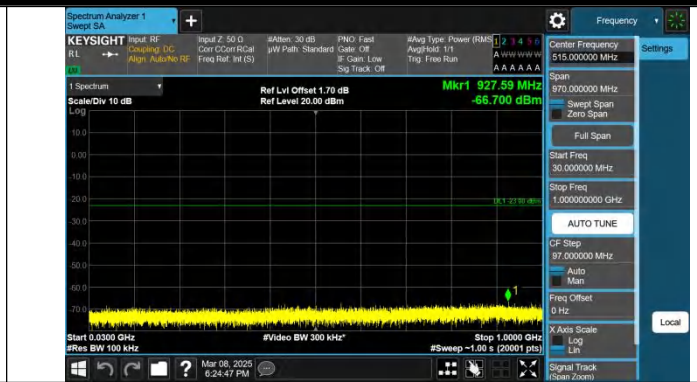
Band25-10MHz-QPSK-26090-1RB#49-30~1000-PASS
