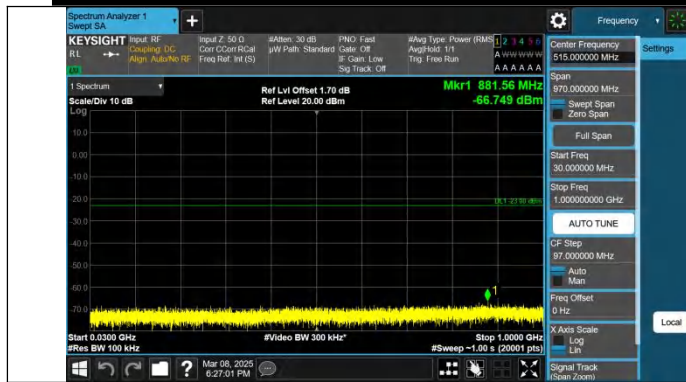
Band25-10MHz-QPSK-26640-1RB#0-30~1000-PASS
