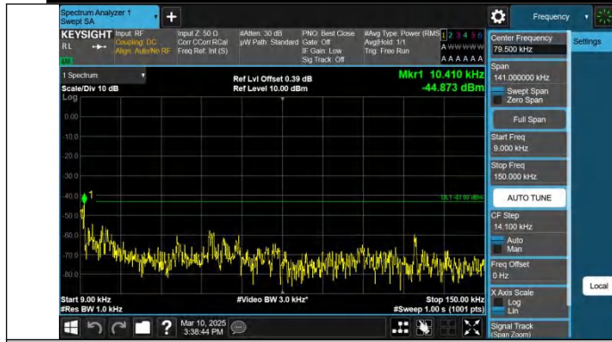
Band25-3MHz-QPSK-26365-1RB#0-0.009~0.15-PASS
