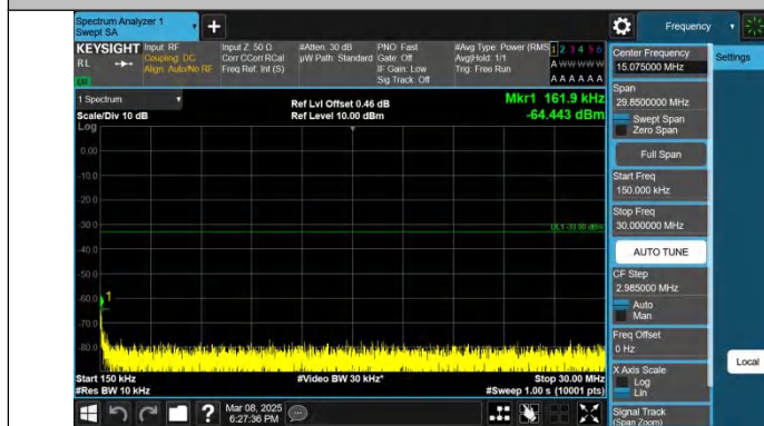
Band25-10MHz-QPSK-26640-1RB#49-0.15~30-PASS
