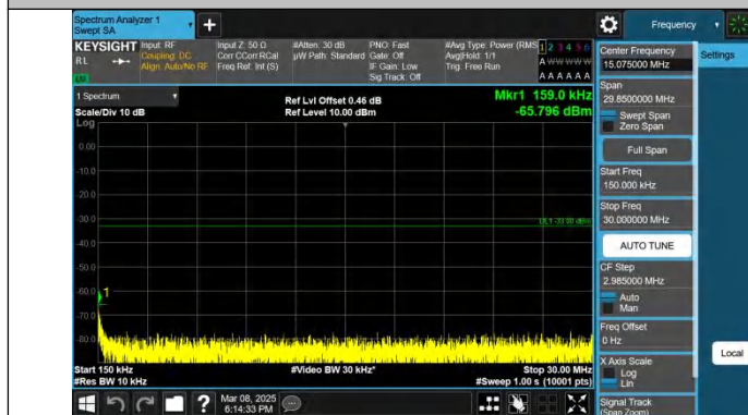
Band25-5MHz-QPSK-26065-1RB#24-0.15~30-PASS
