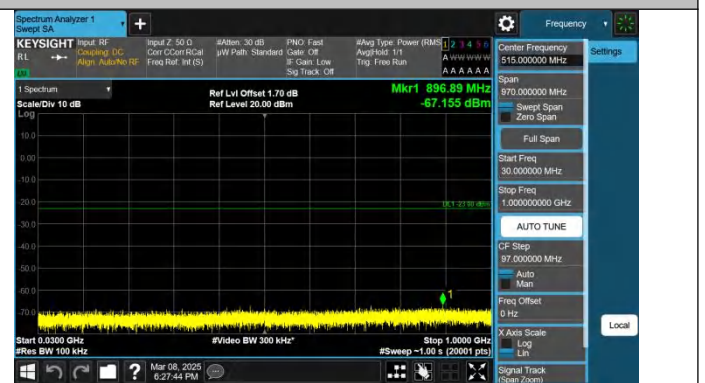
Band25-10MHz-QPSK-26640-1RB#49-30~1000-PASS
