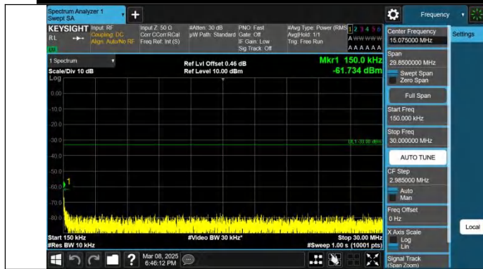
Band25-20MHz-QPSK-26590-1RB#99-0.15~30-PASS
