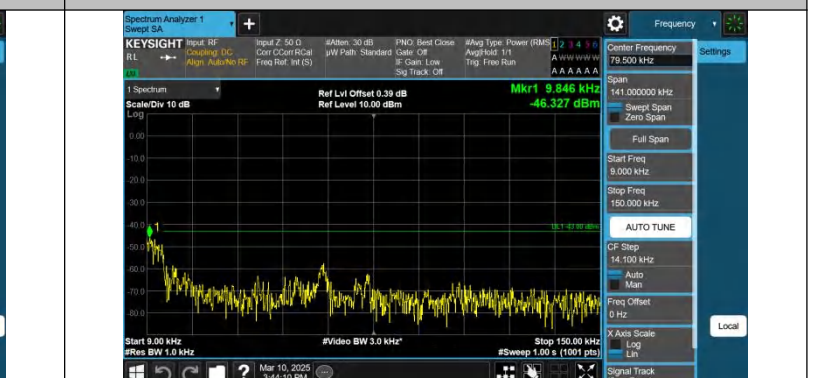
Band25-20MHz-QPSK-26590-1RB#99-0.009~0.15-PASS
