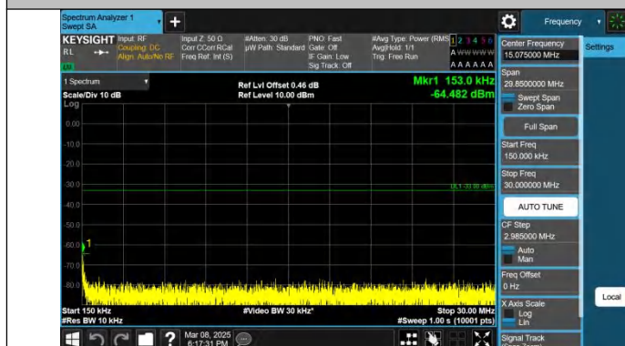
Band25-5MHz-QPSK-26665-1RB#24-0.15~30-PASS
