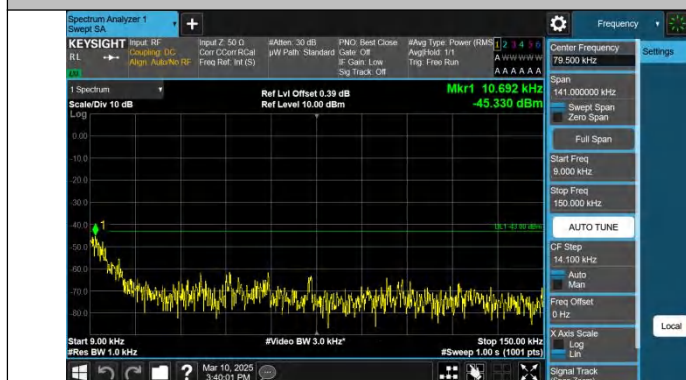
Band25-5MHz-QPSK-26365-1RB#0-0.009~0.15-PASS
