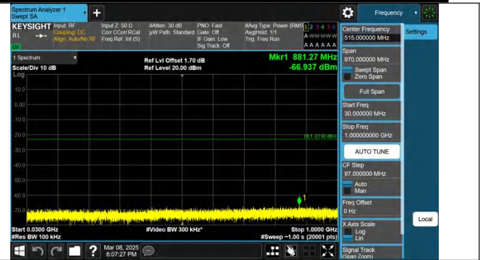
Band25-3MHz-QPSK-26675-1RB#14-30~1000-PASS
