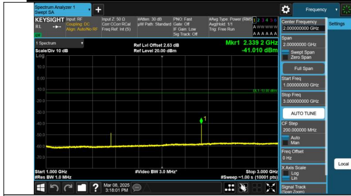
Band13-5MHz-QPSK-23230-1RB#0-1000~3000-PASS
