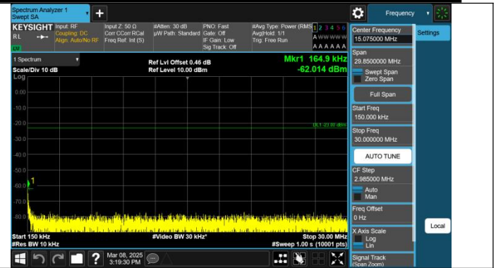
Band13-5MHz-QPSK-23255-1RB#0-0.15~30-PASS
