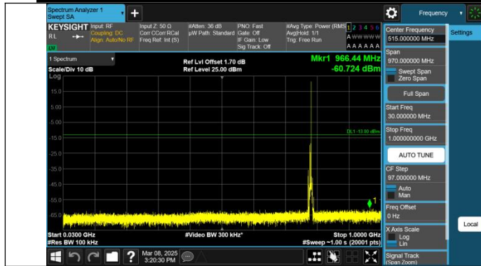
Band13-5MHz-QPSK-23255-1RB#24-30~1000-PASS
