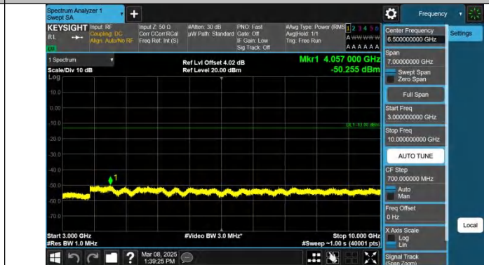
Band12-3MHz-QPSK-23165-1RB#14-3000~10000-PASS
