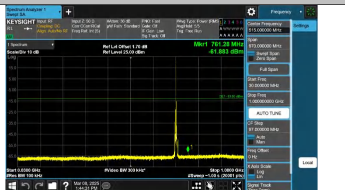
Band12-5MHz-QPSK-23095-1RB#24-30~1000-PASS
