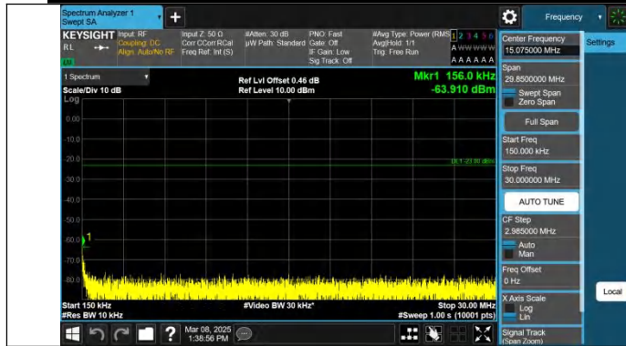
Band12-3MHz-QPSK-23165-1RB#14-0.15~30-PASS
