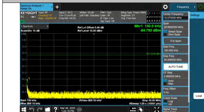
Band12-5MHz-QPSK-23095-1RB#24-0.15~30-PASS
