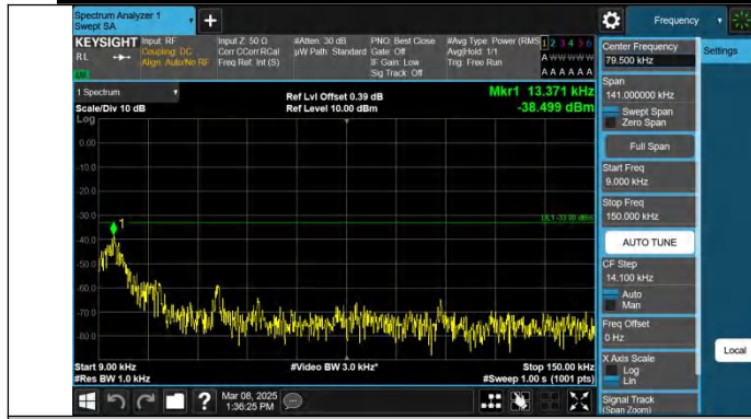
Band12-3MHz-QPSK-23095-1RB#0-0.009~0.15-PASS
