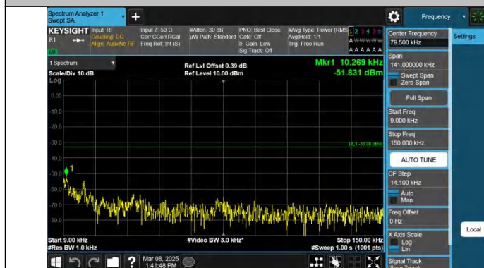
Band12-5MHz-QPSK-23035-1RB#0-0.009~0.15-PASS
