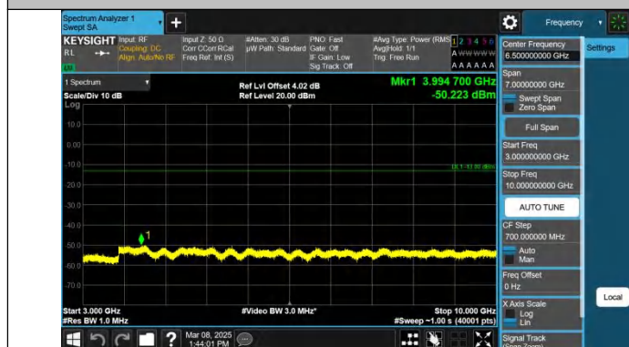
Band12-5MHz-QPSK-23095-1RB#0-3000~10000-PASS
