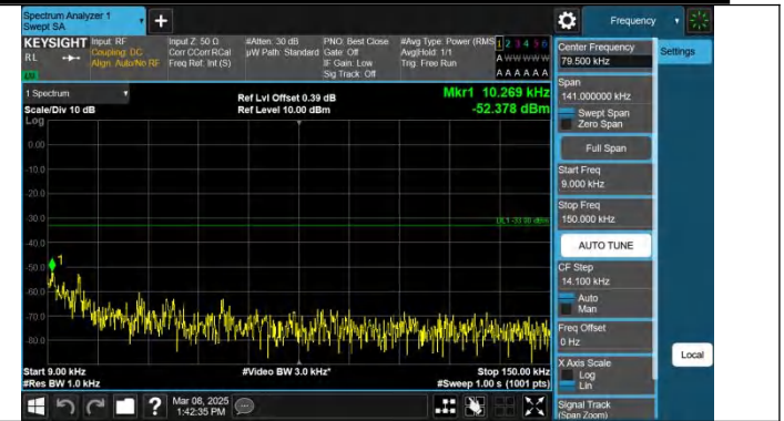
Band12-5MHz-QPSK-23035-1RB#24-0.009~0.15-PASS
