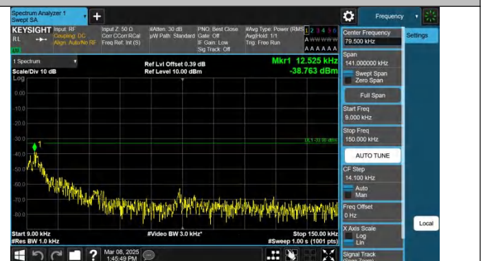
Band12-5MHz-QPSK-23155-1RB#24-0.009~0.15-PASS
