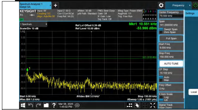
Band12-5MHz-QPSK-23155-1RB#0-0.009~0.15-PASS
