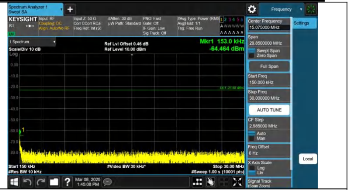
Band12-5MHz-QPSK-23155-1RB#0-0.15~30-PASS
