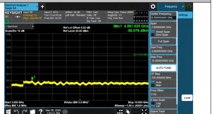
Band12-10MHz-QPSK-23130-1RB#49-3000~10000-PASS
