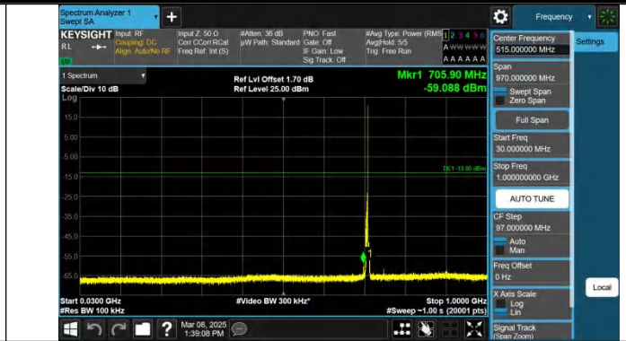
Band12-3MHz-QPSK-23165-1RB#14-30~1000-PASS
