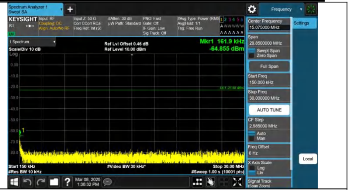
Band12-3MHz-QPSK-23095-1RB#0-0.15~30-PASS
