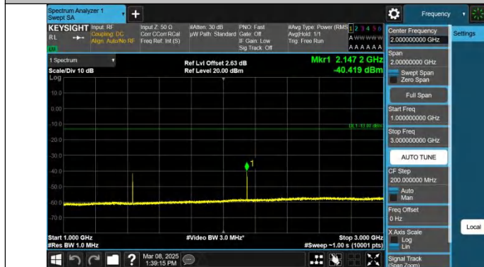
Band12-3MHz-QPSK-23165-1RB#14-1000~3000-PASS
