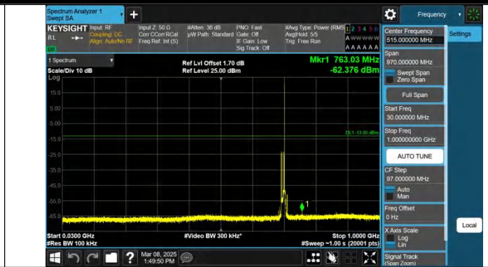
Band12-10MHz-QPSK-23060-1RB#49-30~1000-PASS
