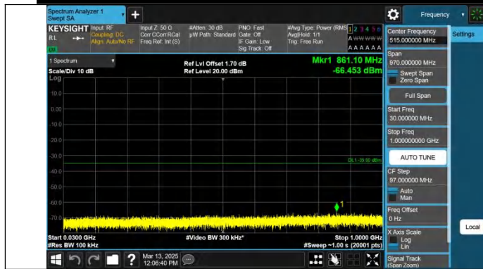
Band7-20MHz-QPSK-21350-1RB#0-30~1000-PASS
