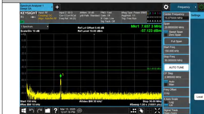
Band7-20MHz-QPSK-21350-1RB#99-0.15~30-PASS
