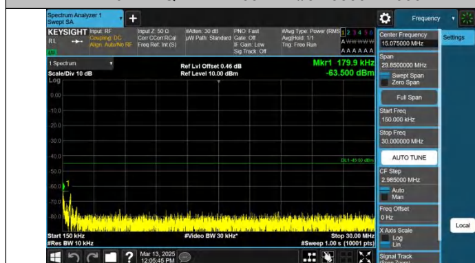
Band7-20MHz-QPSK-21100-1RB#99-0.15~30-PASS
