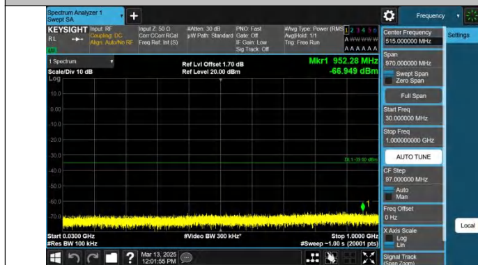
Band7-15MHz-QPSK-21375-1RB#0-30~1000-PASS
