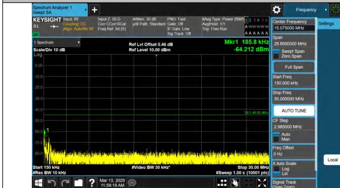
Band7-15MHz-QPSK-20825-1RB#74-0.15~30-PASS
