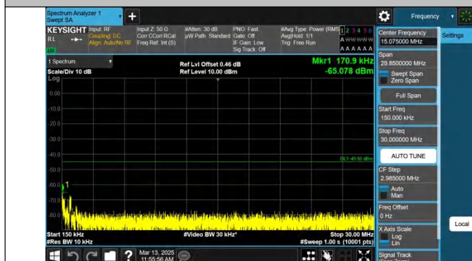
Band7-10MHz-QPSK-21100-1RB#49-0.15~30-PASS
