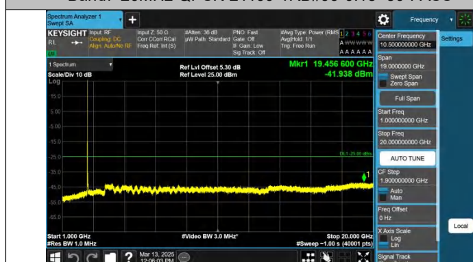
Band7-20MHz-QPSK-21100-1RB#99-1000~20000-PASS
