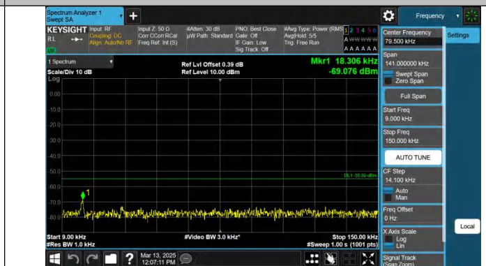
Band7-20MHz-QPSK-21350-1RB#99-0.009~0.15-PASS
