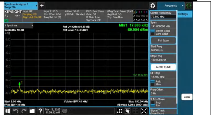
Band7-15MHz-QPSK-20825-1RB#74-0.009~0.15-PASS
