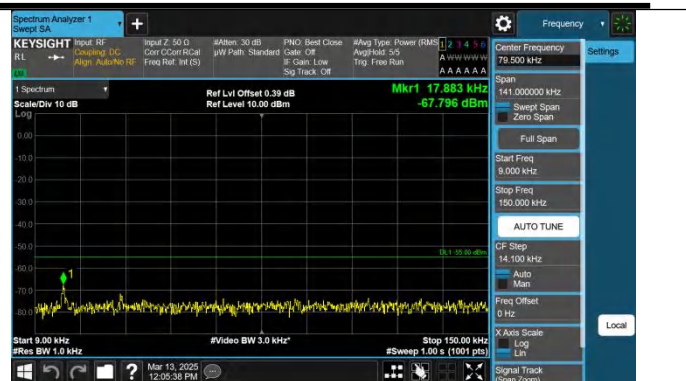
Band7-20MHz-QPSK-21100-1RB#99-0.009~0.15-PASS
