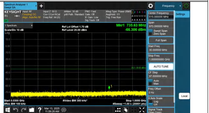
Band7-15MHz-QPSK-20825-1RB#74-30~1000-PASS
