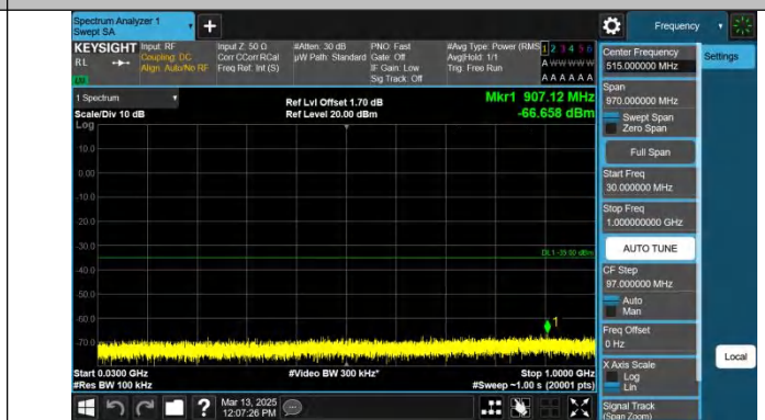
Band7-20MHz-QPSK-21350-1RB#99-30~1000-PASS
