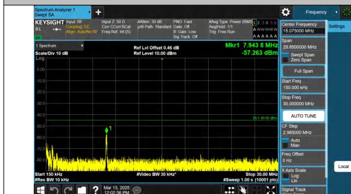
Band7-15MHz-QPSK-21375-1RB#74-0.15~30-PASS
