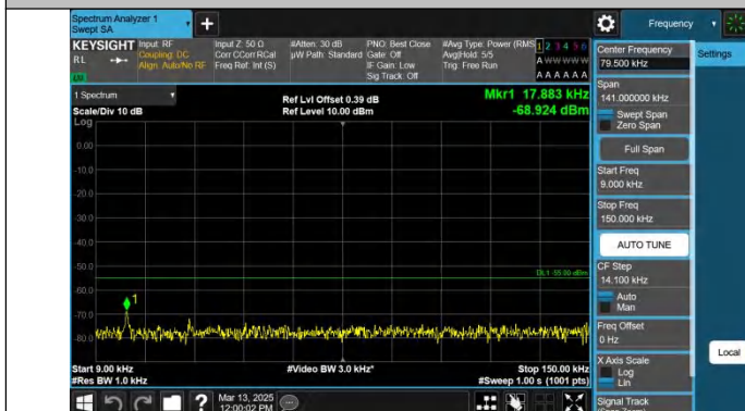
Band7-15MHz-QPSK-21100-1RB#0-0.009~0.15-PASS
