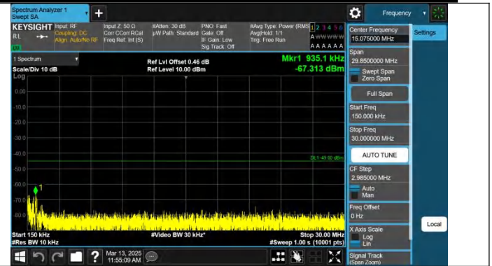
Band7-10MHz-QPSK-21100-1RB#0-0.15~30-PASS
