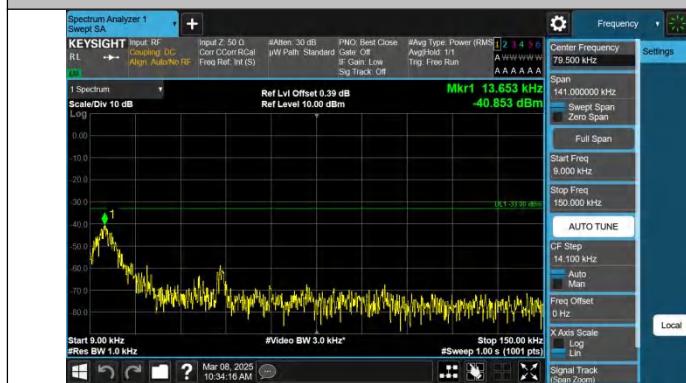
Band5-5MHz-QPSK-20425-1RB#0-0.009~0.15-PASS
