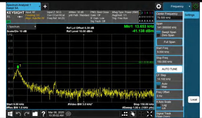
Band5-5MHz-QPSK-20425-1RB#24-0.009~0.15-PASS
