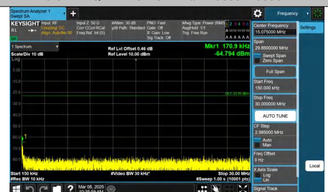
Band5-5MHz-QPSK-20525-1RB#0-0.15~30-PASS
