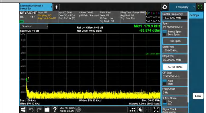
Band5-5MHz-QPSK-20425-1RB#0-0.15~30-PASS
