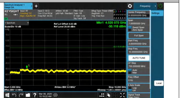
Band5-1.4MHz-QPSK-20643-1RB#5-3000~10000-PASS
