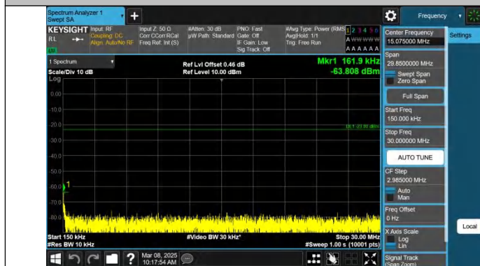
Band5-1.4MHz-QPSK-20643-1RB#5-0.15~30-PASS
