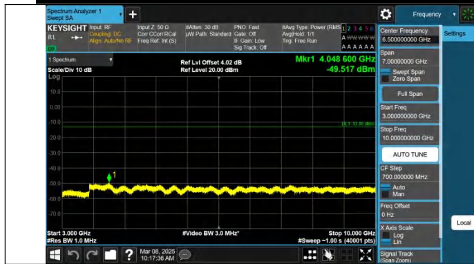
Band5-1.4MHz-QPSK-20643-1RB#0-3000~10000-PASS
