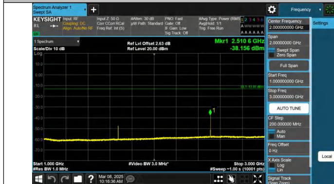
Band5-1.4MHz-QPSK-20525-1RB#5-1000~3000-PASS
