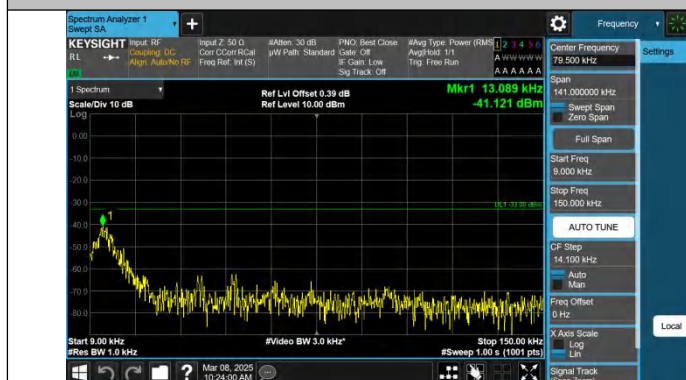
Band5-3MHz-QPSK-20415-1RB#0-0.009~0.15-PASS
