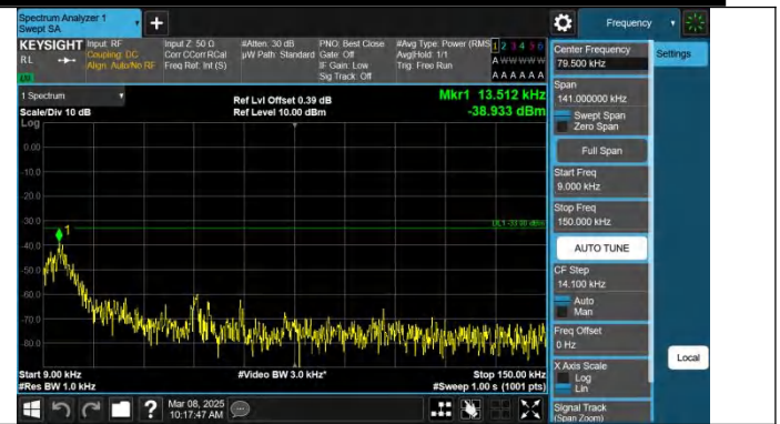
Band5-1.4MHz-QPSK-20643-1RB#5-0.009~0.15-PASS
