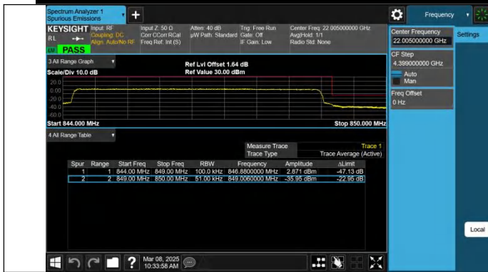
Band5-5MHz-QPSK-20625-25RB#0-PASS
