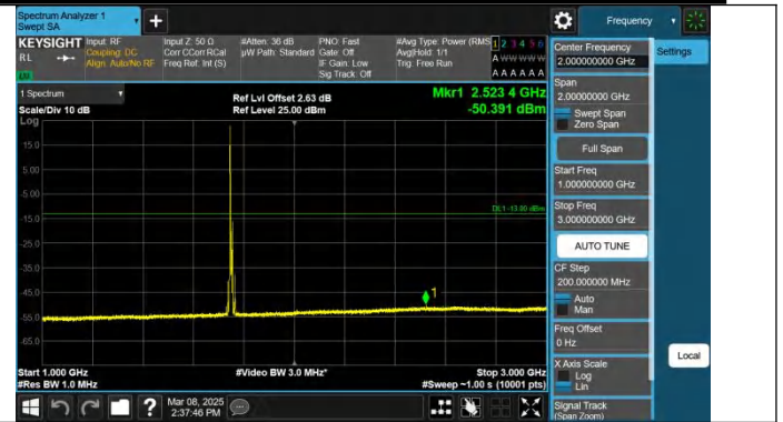
Band4-10MHz-QPSK-20350-1RB#0-1000~3000-PASS
