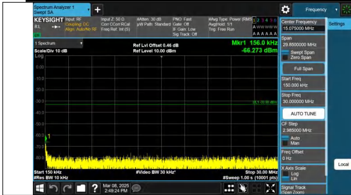
Band4-15MHz-QPSK-20175-1RB#74-0.15~30-PASS
