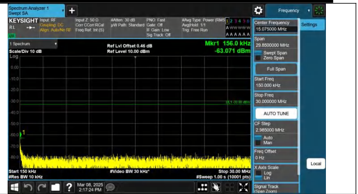
Band4-5MHz-QPSK-20375-1RB#0-0.15~30-PASS
