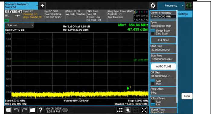
Band4-10MHz-QPSK-20000-1RB#49-30~1000-PASS
