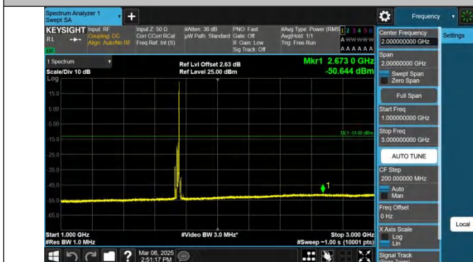
Band4-15MHz-QPSK-20325-1RB#74.1000~3000-PASS
