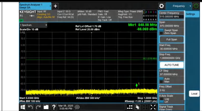
Band4-20MHz-QPSK-20300-1RB#99-30~1000-PASS
