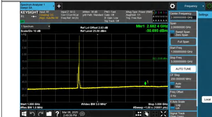
Band4-15MHz-QPSK-20175-1RB#74-1000~3000-PASS
