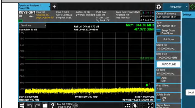
Band4-10MHz-QPSK-20000-1RB#0-30~1000-PASS
