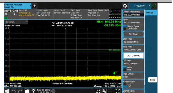
Band4-5MHz-QPSK-20375-1RB#24-30~1000-PASS
