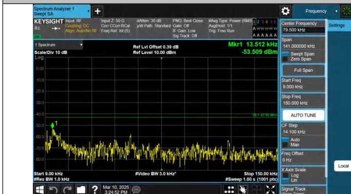
Band4-15MHz-QPSK-20325-1RB#0-0.009~0.15-PASS
