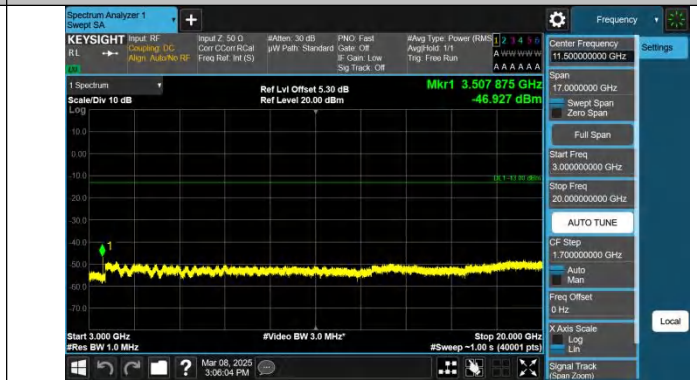
Band4-20MHz-QPSK-20300-1RB#99-3000~20000-PASS
