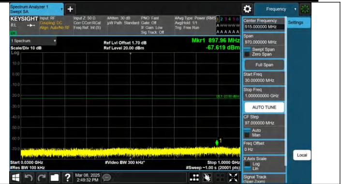
Band4-15MHz-QPSK-20175-1RB#74-30~1000-PASS
