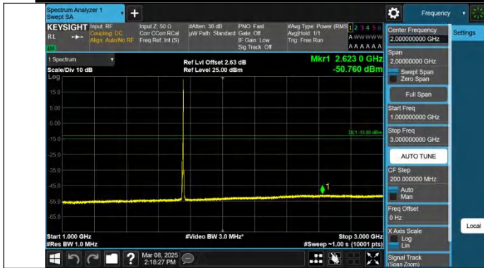
Band4-5MHz-QPSK-20375-1RB#24-1000~3000-PASS
