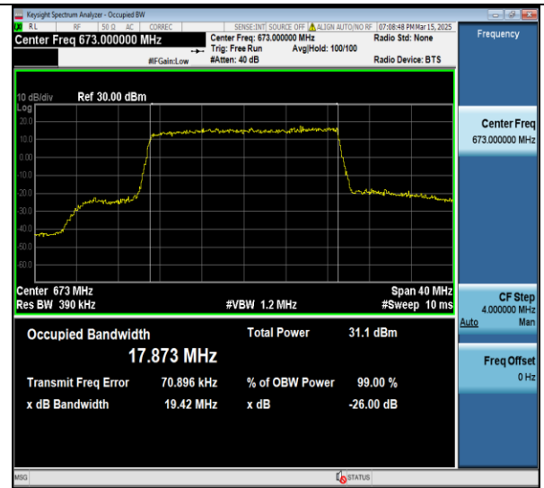
Band71-20MHz-16QAM-133222-100RB#0-PASS
