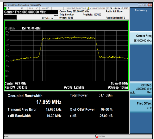
Band71-20MHz-16QAM-133322-100RB#0-PASS
