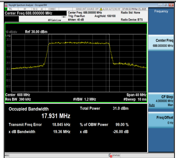
Band71-20MHz-16QAM-133372-100RB#0-PASS
