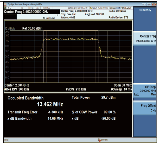
Band41-15MHz-16QAM-39725-75RB#0-PASS
