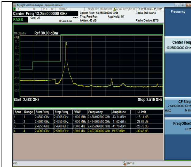
Band41-20MHz-QPSK-39750-1RB#0-PASS
