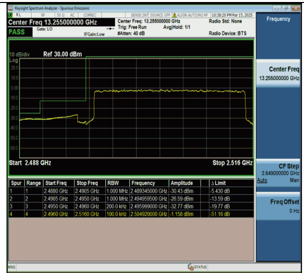
Band41-20MHz-QPSK-39750-100RB#0-PASS
