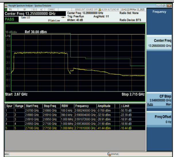
Band41-20MHz-QPSK-41490-100RB#0-PASS
