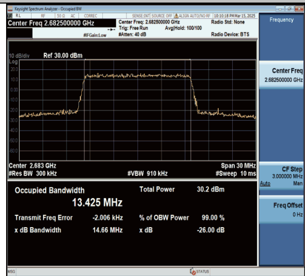
Band41-15MHz-16QAM-41515-75RB#0-PASS
