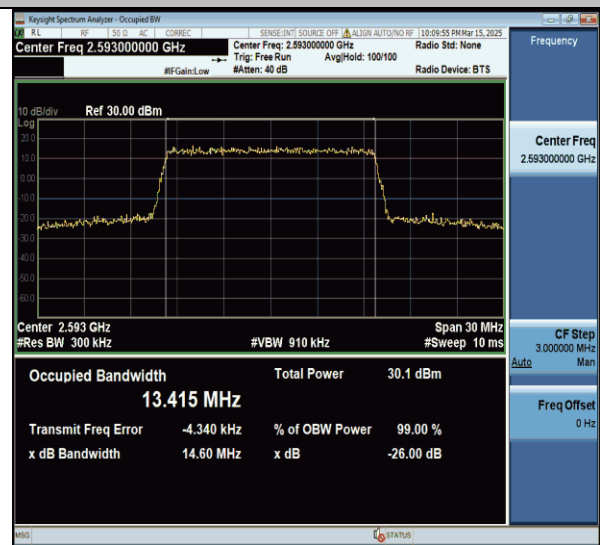
Band41-15MHz-16QAM-40620-75RB#0-PASS
