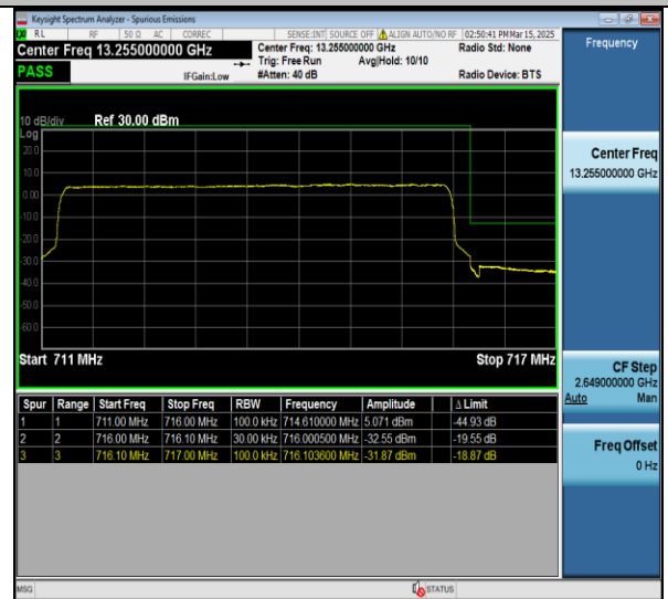
Band12-5MHz-QPSK-23155-25RB#0-PASS
