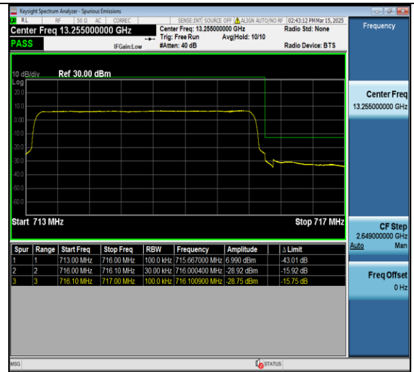
Band12-3MHz-QPSK-23165-15RB#0-PASS
