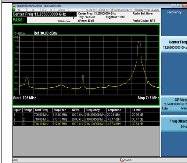
Band12-10MHz-QPSK-23130-1RB#49-PASS
