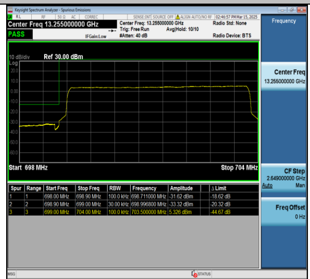
Band12-5MHz-QPSK-23035-25RB#0-PASS
