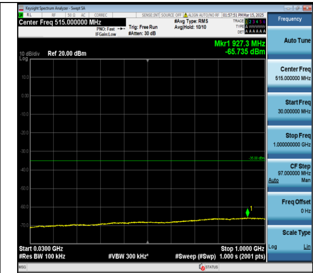
Band7-20MHz-QPSK-21100-1RB#0-30~1000-PASS
