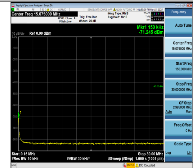
Band7-20MHz-QPSK-21350-1RB#0-0.15~30-PASS
