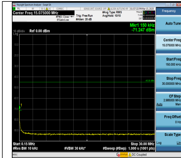
Band7-20MHz-QPSK-21100-1RB#0-0.15~30-PASS
