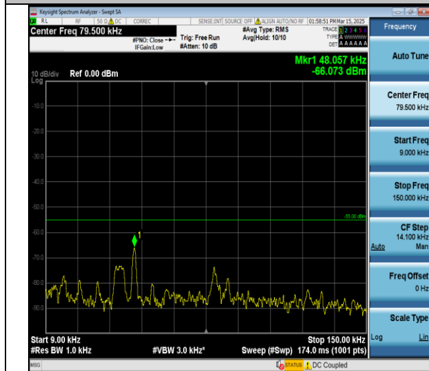
Band7-20MHz-QPSK-21350-1RB#0-0.009~0.15-PASS
