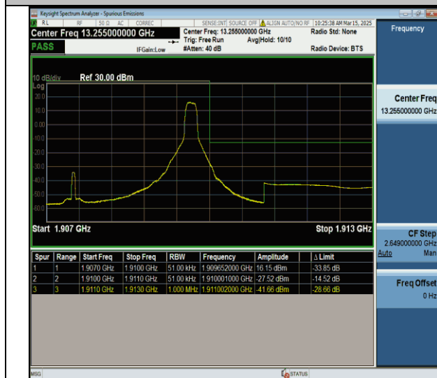
Band2-5MHz-QPSK-19175-1RB#24-PASS
