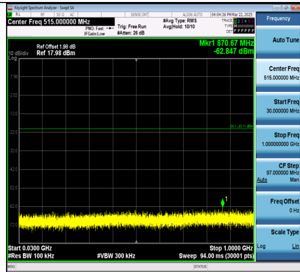
BLE_1M-Ant0-2480-30~1000-PASS
