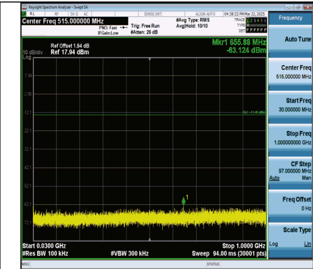
3DH5-Ant0-2402-30~1000-PASS
