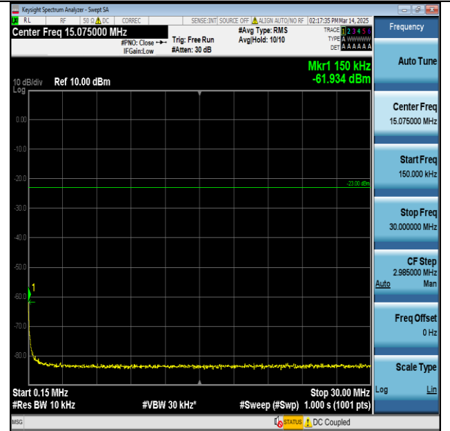
Band71-20MHz-QPSK-133372-1RB#0-0.15~30-PASS
