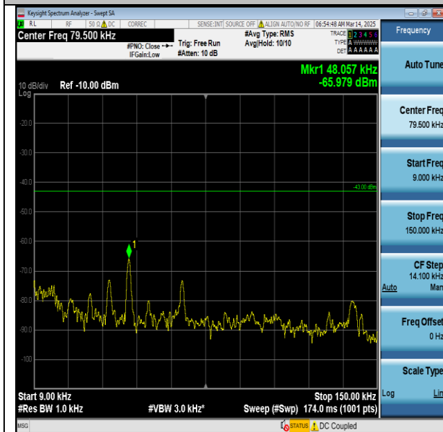
Band4-20MHz-QPSK-20300-1RB#0-0.009~0.15-PASS
