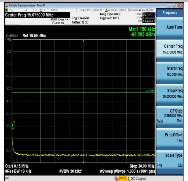
Band4-20MHz-QPSK-20300-1RB#0-0.15~30-PASS
